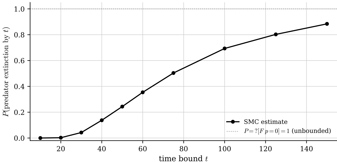
Lotka-Volterra CTMC: bounded extinction probability
