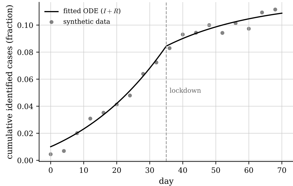
Pisa-style ODE fit (first 70 days)
