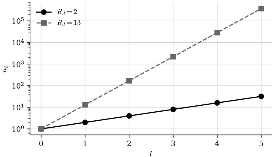
Exponential growth ( n_0 = 1 )
