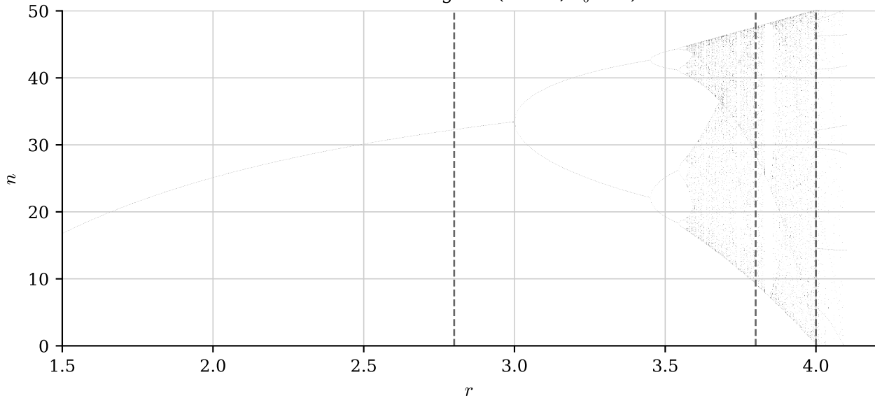
Bifurcation diagram ( K = 50 , n_0 = 10 )
