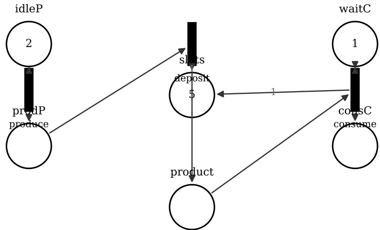
Producer-consumer (capacity 5)
