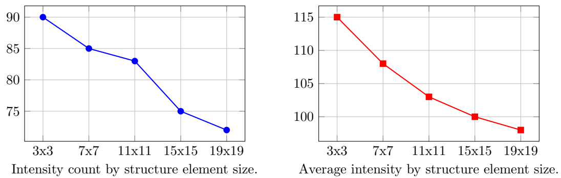
Figure 1: Plot of the number of unique intensities (left) and the average pixel intensity (right) of Grayscale Erosion applied with increasing structure element sizes.
