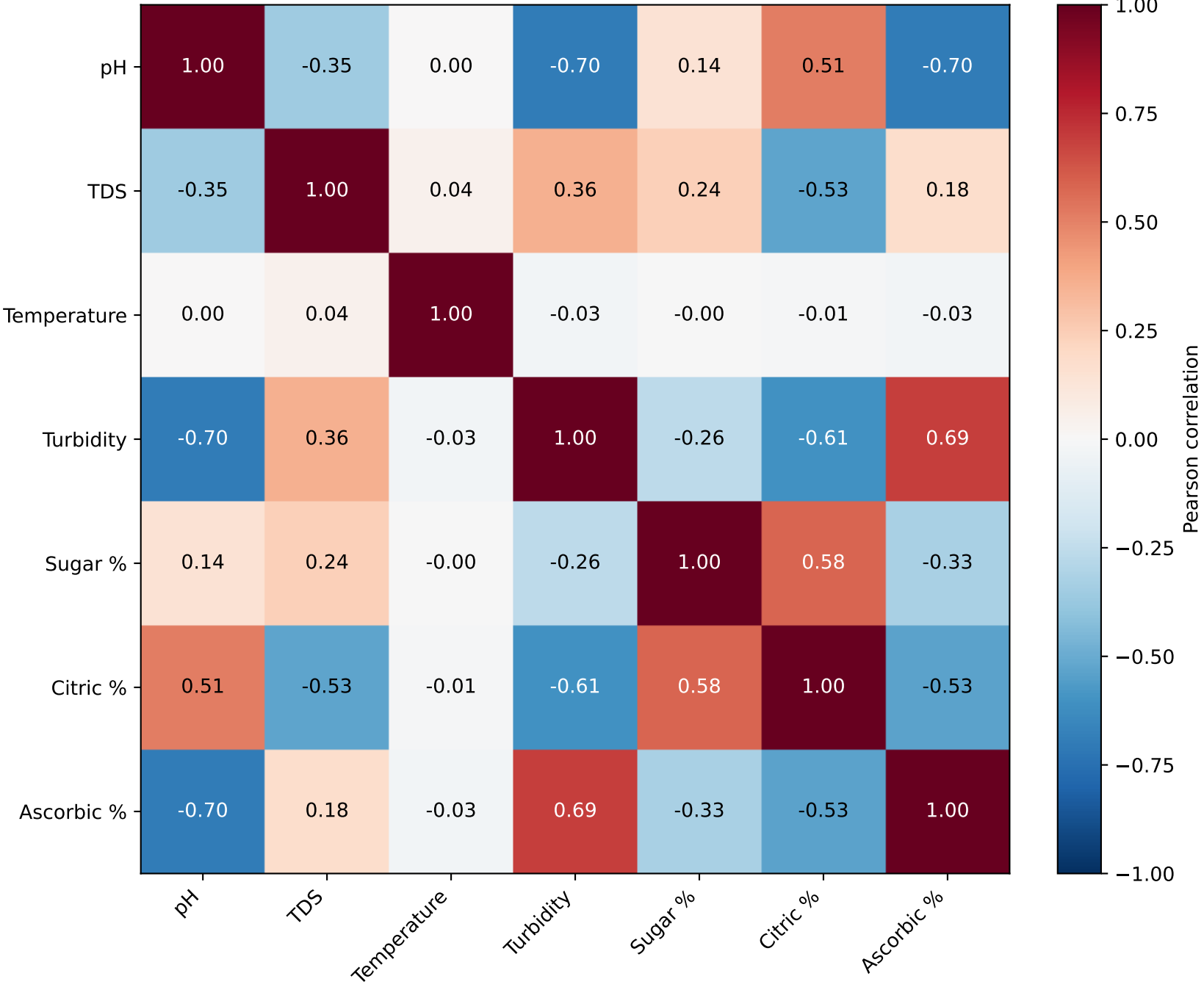
Correlation Matrix: Sensor Features vs Composition Targets
