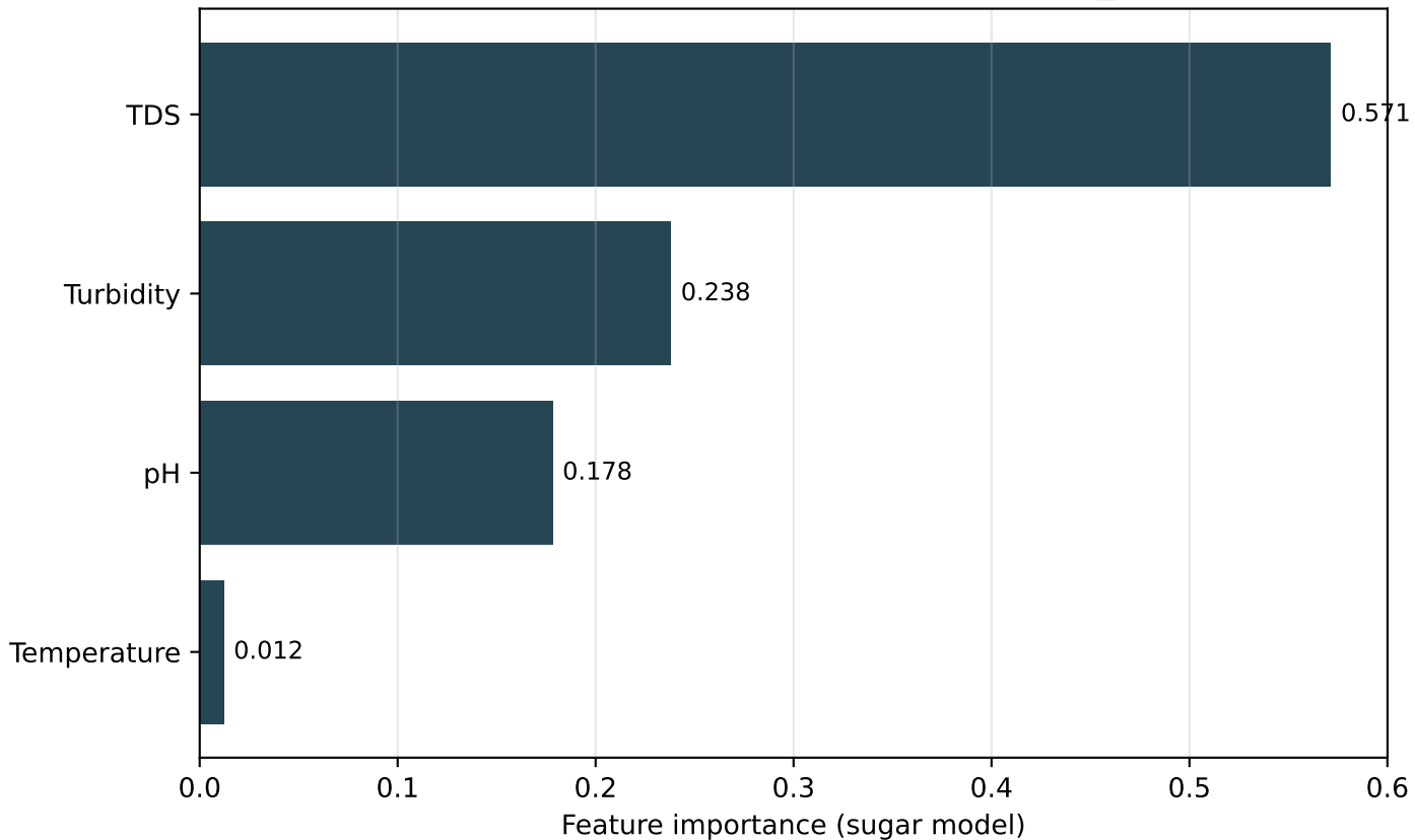
Figure: Random Forest Feature Importance (ML_2 Sugar)
