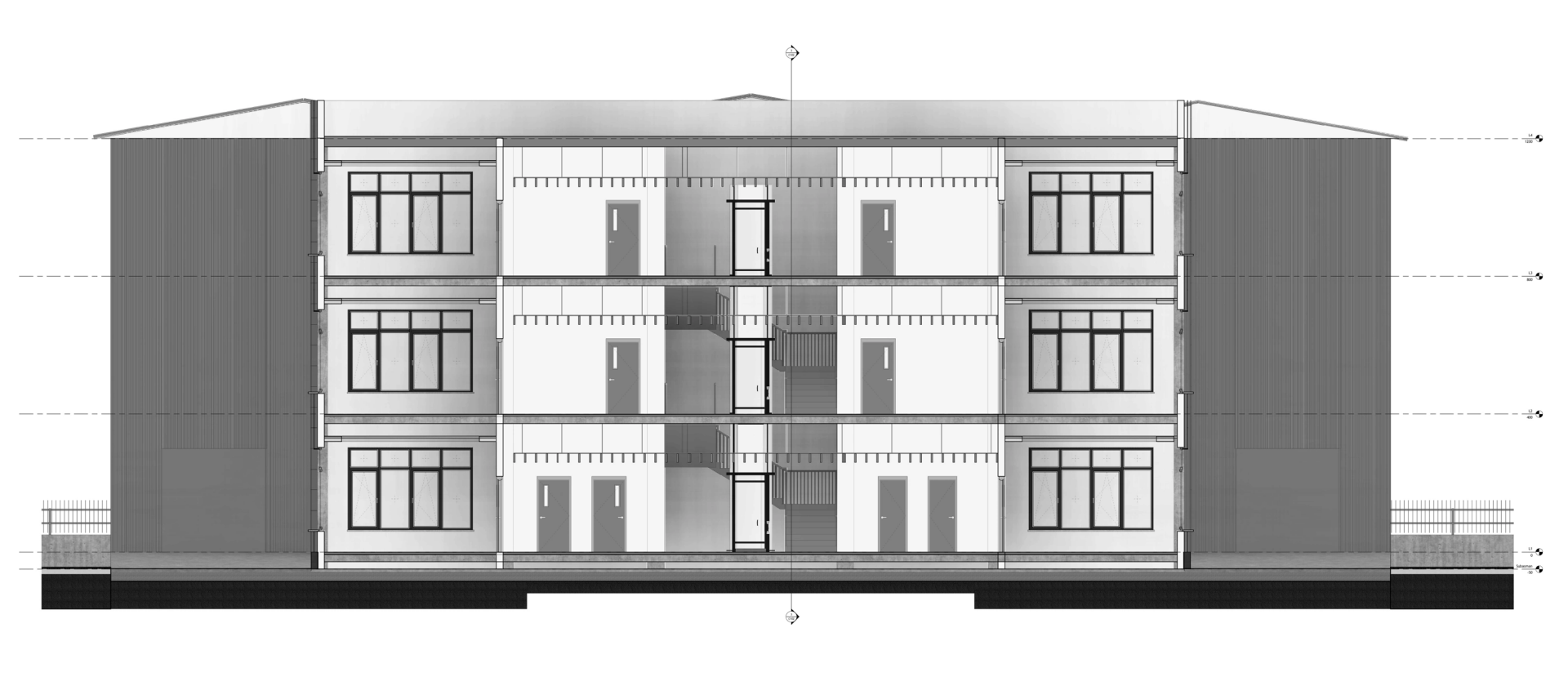
02 / FACADE ELEVATION
