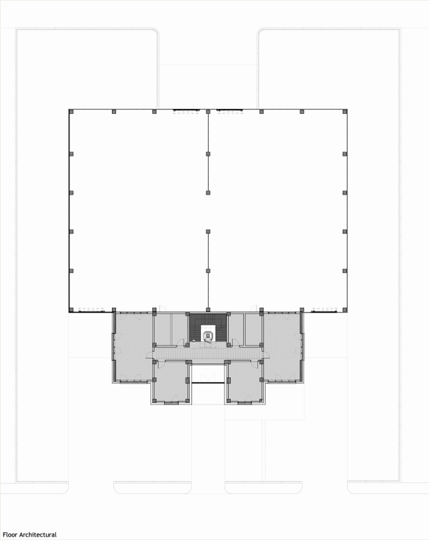
03 / FLOOR PLAN
