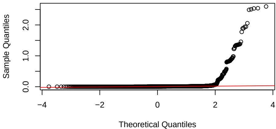
Q-Q Original
