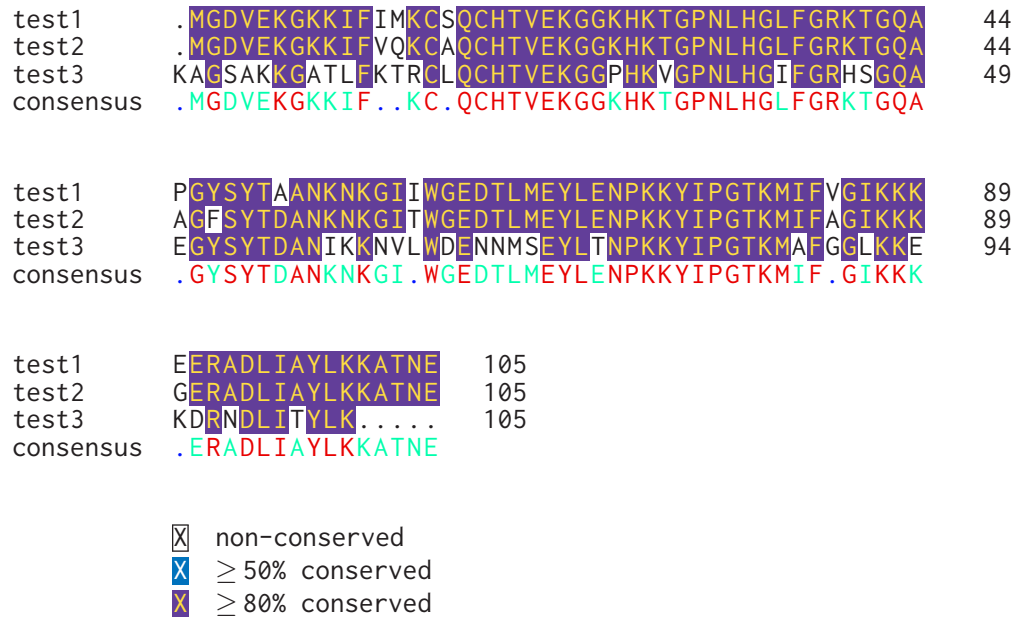
Figure 2: Alignment using Clustal Omega and Identity mode in texshade
