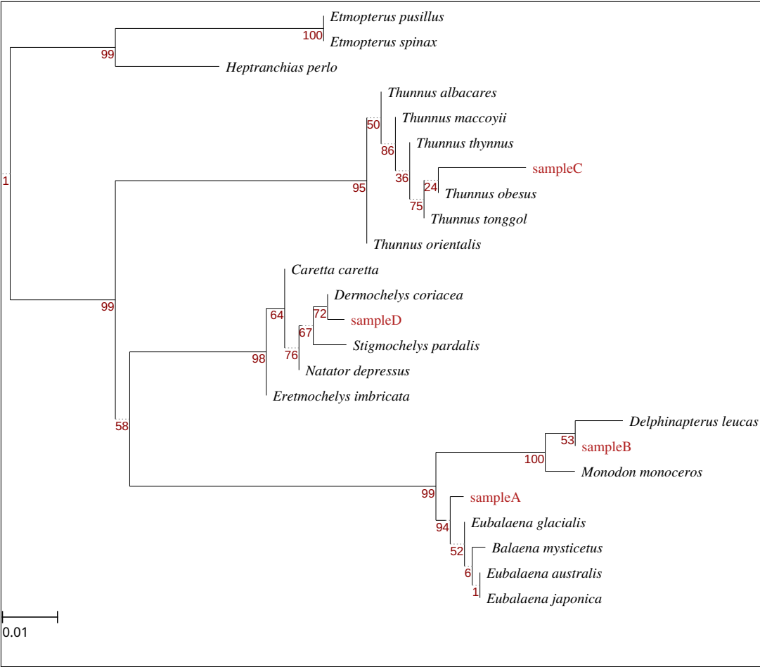
Figure 5: Phylogenetic tree resulting from Fig. 4 alignment.
