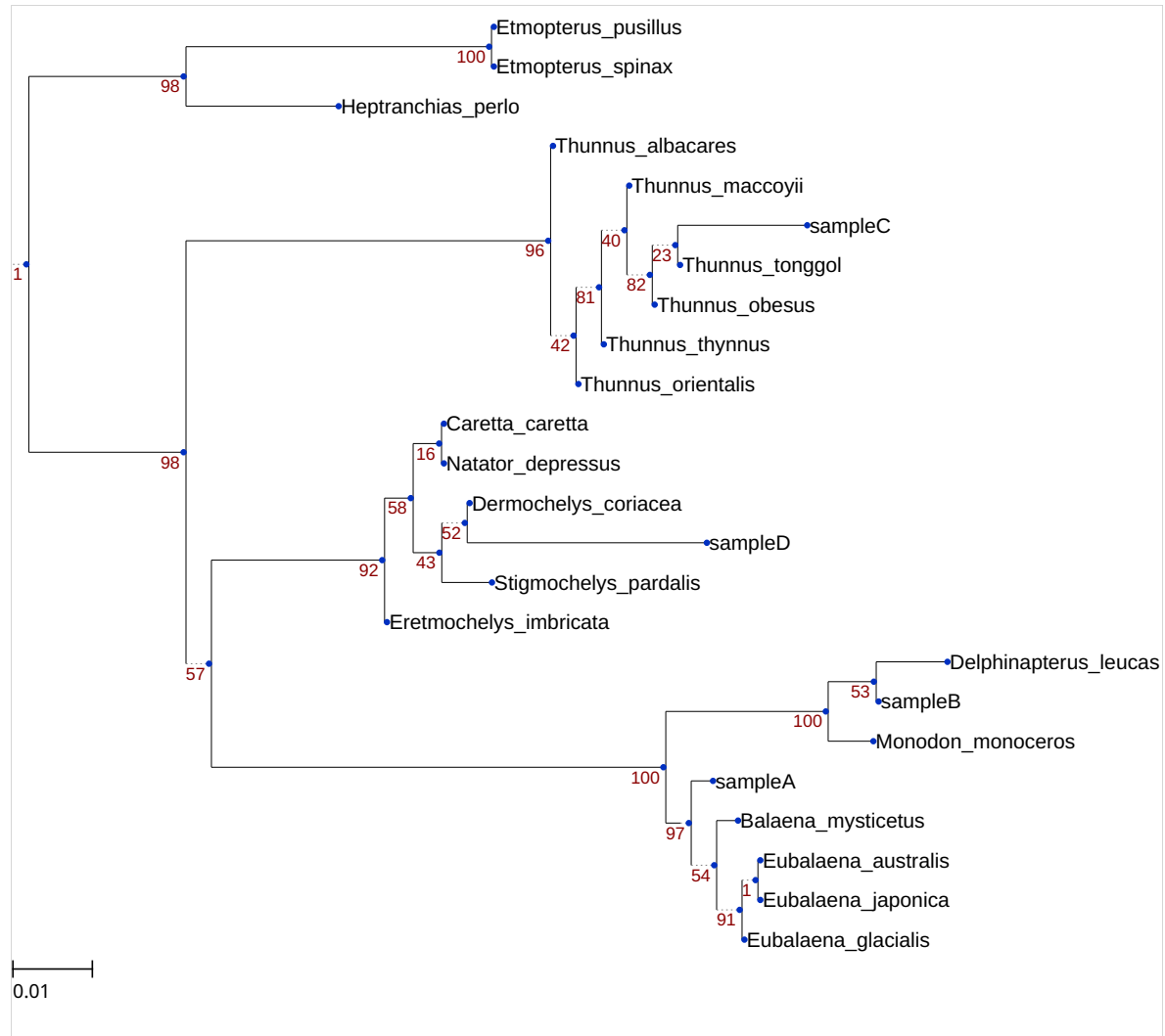
Figure 1: Maximum-likelihood phylogenetic tree with placement of unknown meat samples and their top BLAST hits
