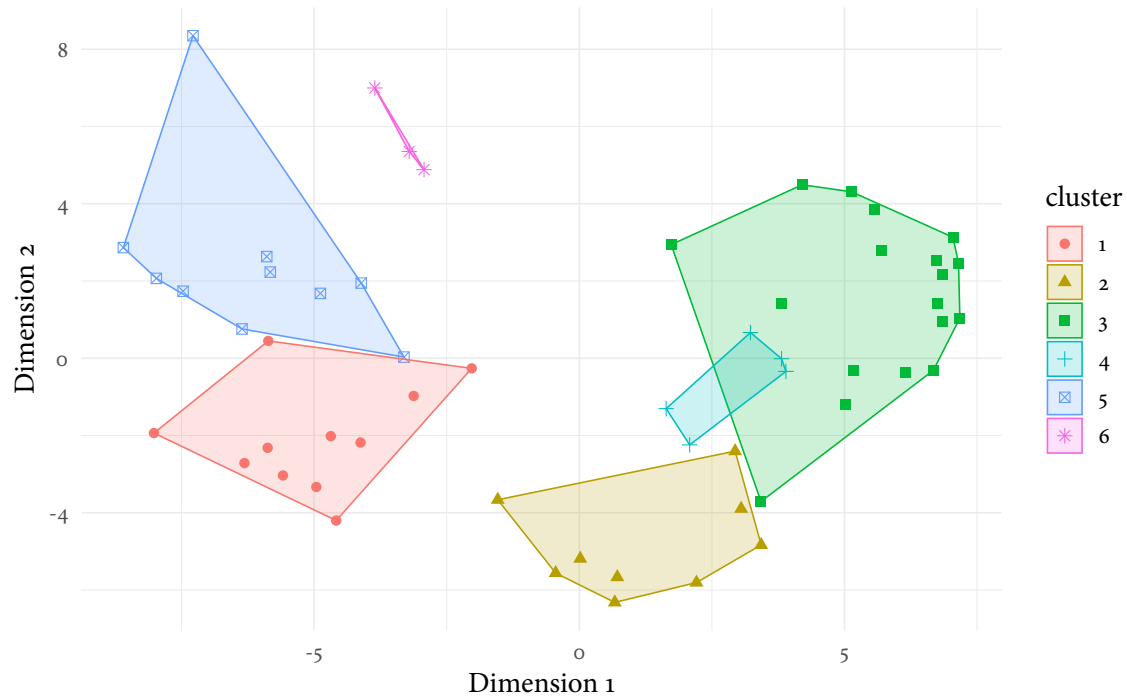
Cluster plot
