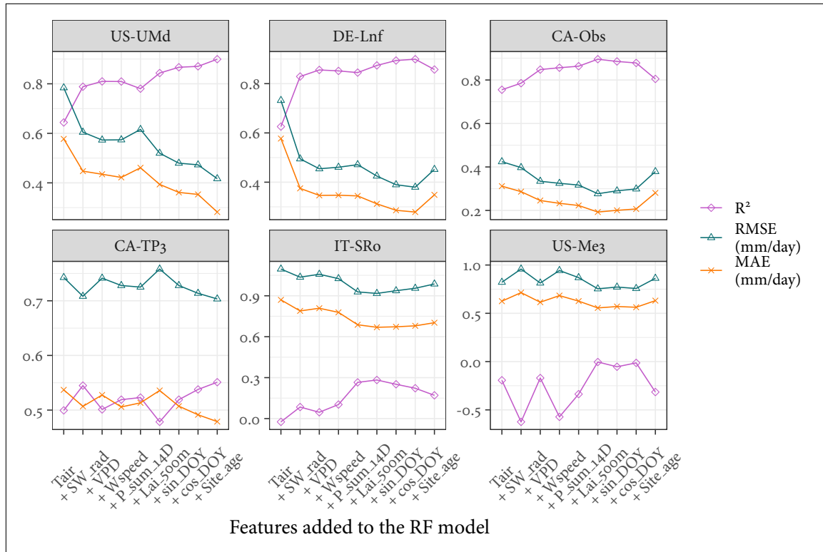
Figure 6: R^2 , RMSE, and MAE for medoid cluster site predictions of daily ET during sensitivity testing (ordered left-right and top-bottom by peak R^2 ). Models were built and tested using a consecutively greater number of input features from FLUXNET and LAI data (for example, the ‘+VPD model’ incorporates Tair, SW_rad, and VPD as training and input features). R^2 performance at only half of the sites was moderate or strong, and suggests that adding features up to LAI improved prediction accuracy at four of the six medoid sites. Adding site age as a final feature led to mixed performance across ET predictions made at medoid sites, with only two of the six benefiting in terms of predictive performance from this input feature.
