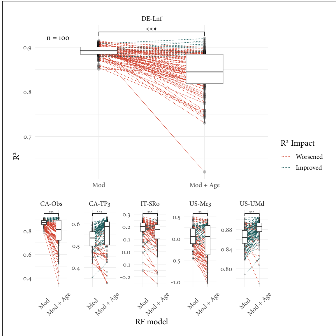
Figure 7: Paired box-plots indicate the impact on R^2 when age is added as a feature to RF models across 100 repeated runs of randomly sampled training datasets. Points are connected on a per-run basis where training dataset site composition is identical. Wilcoxon signed-rank tests suggest model performances differ significantly at all test sites, as indicated by the significance annotation on each facet (***) signifies p < 0.001 , ** signifies p < 0.01 [8]). DE-Lnf is shown large for readability as an example, with other cluster medoid sites shown at a reduced scale for comparison.
