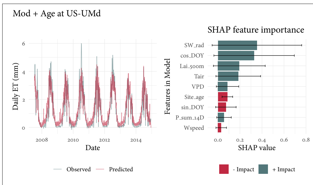
(b) Time series observed daily ET overlaid with the predicted daily ET using the 'Mod + Age' RF model seen on the left, with average SHAP feature importance values across all predictions made with this model on the right. Time series plot suggests a strong fit to the observed data but with peak ET rates in extreme summers being under-predicted, in line with the shape seen in plot a. Feature importance with SHAP...[CONTINUE]
