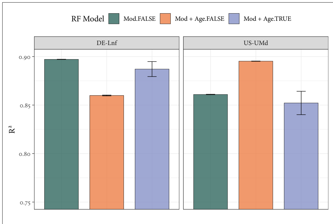
Figure 3: Bar plot showing the effect of different model setups on R^2 at DE-Lnf and US-UMd, with error bars indicating standard error. Models were trained using a leave one group out (LOGO) approach, with ten repeats using different NumPy seeds. To assess whether site age was acting as a proxy for other site-level characteristics in these models, a model which randomly shuffled ages between sites was also formed using identical seeds and LOGO approach. This ‘shuffled age’ model appeared to increase R^2 at DE-Lnf compared to the Mod + Age model where an opposite effect was observed at US-UMd, suggesting that true age-ET relationships learned by the model transfer well to predicting ET at US-UMd, but not at DE-Lnf.
