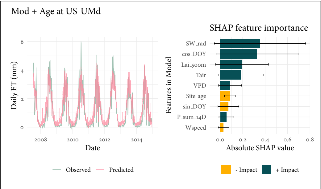
(a) Time series observed daily ET overlaid with the predicted daily ET using the ‘Mod + Age’ RF model seen on the left, with average SHAP feature importance values across all predictions made with this model on the right. Time series plot suggests a strong fit to the observed data but with peak ET rates in extreme summers being under-predicted, in line with the shape seen in plot a. Feature importance with SHAP...[CONTINUE]
