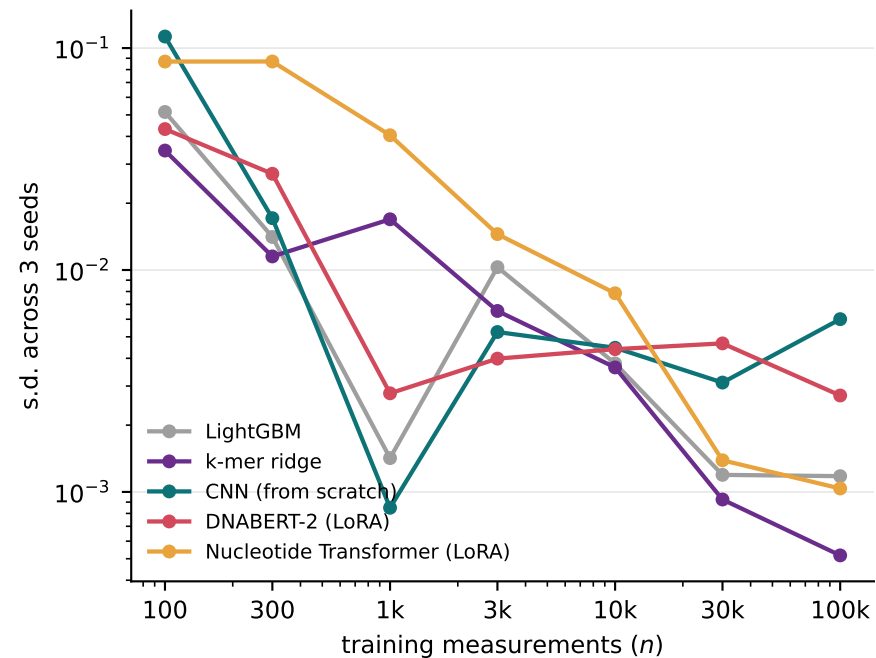
A Reliability collapses at small n
