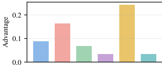
Planning L2
