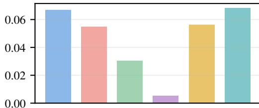
Motion ADE
