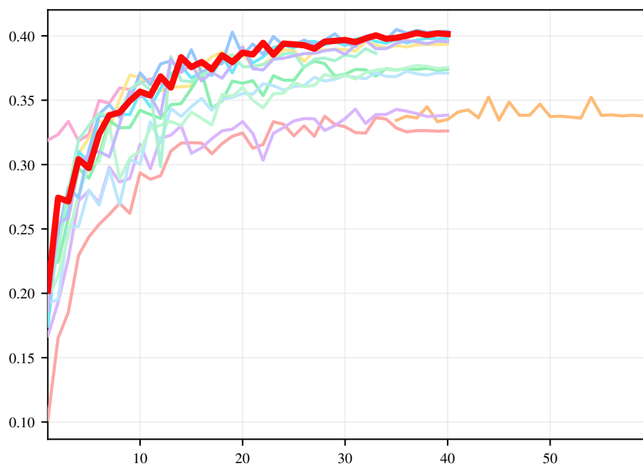
Detection NDS
