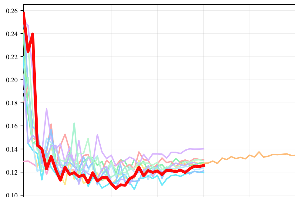
Motion MR
