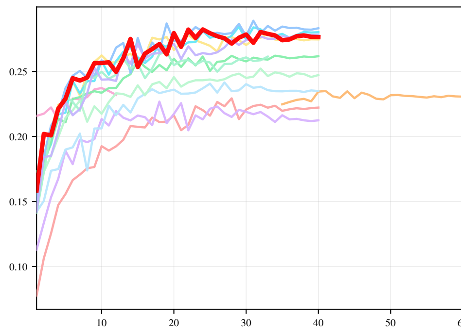
Detection mAP
