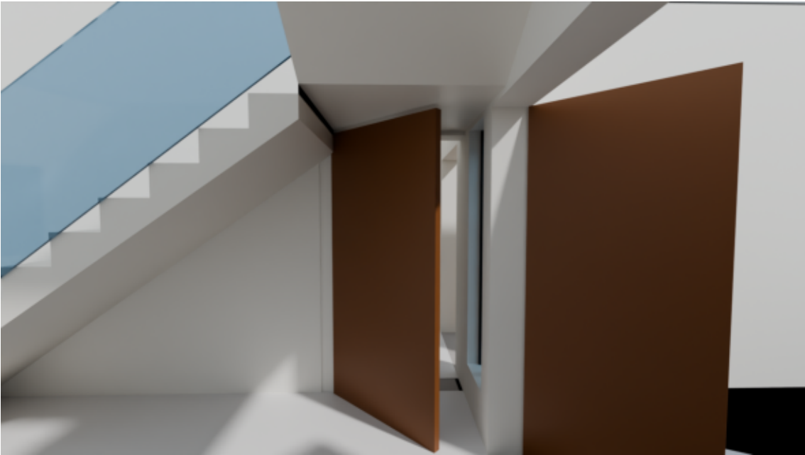
FROM THE FOYER LOOKING EAST - lobby door D8 (open), drawing door & washroom beyond
