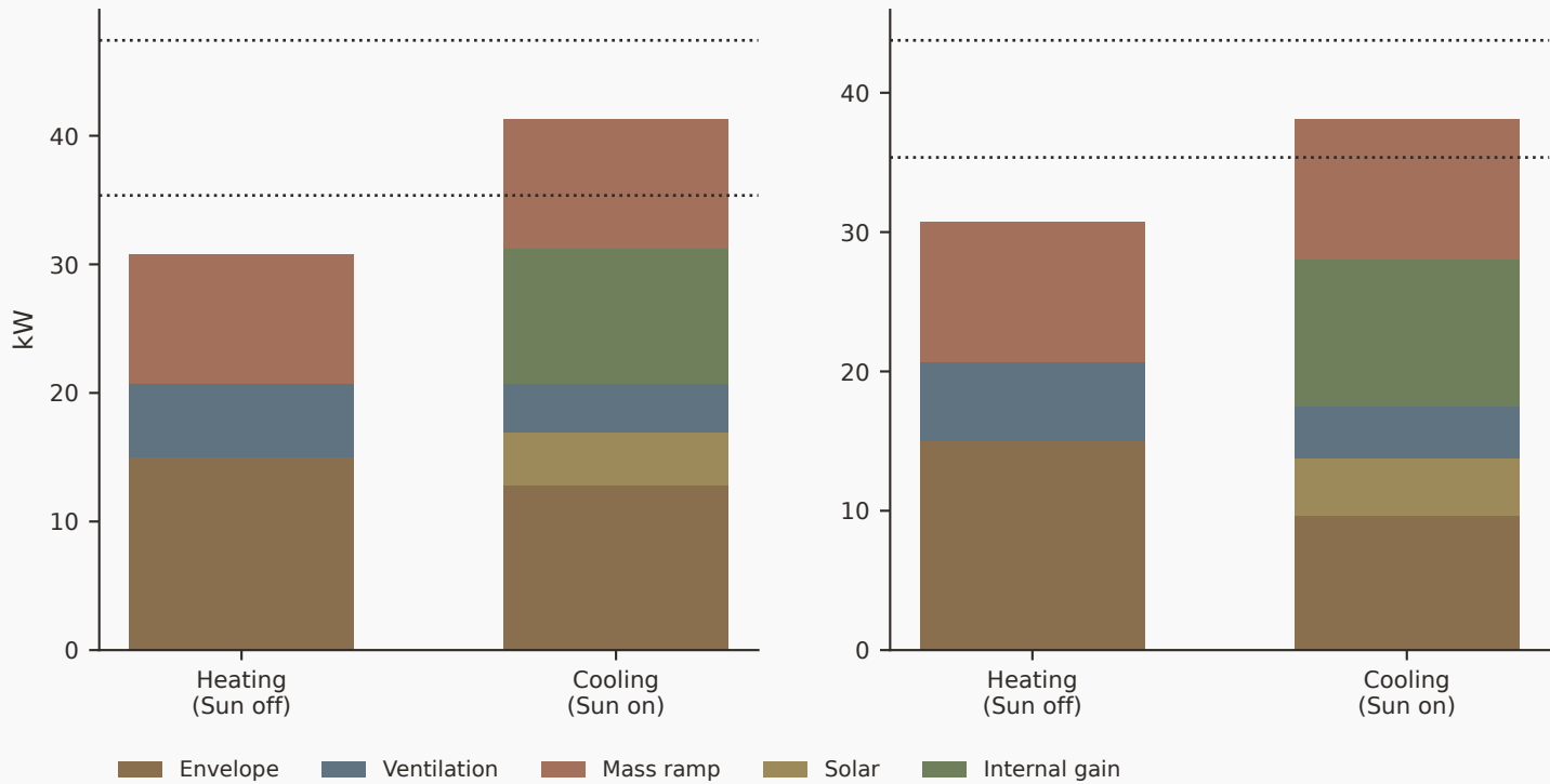
Climate chamber worst case — design capacity by component (dotted line = design total incl. margin) Boundary summer 45°C (confirmed design condition) Boundary summer 32°C (historical reference, superseded)
