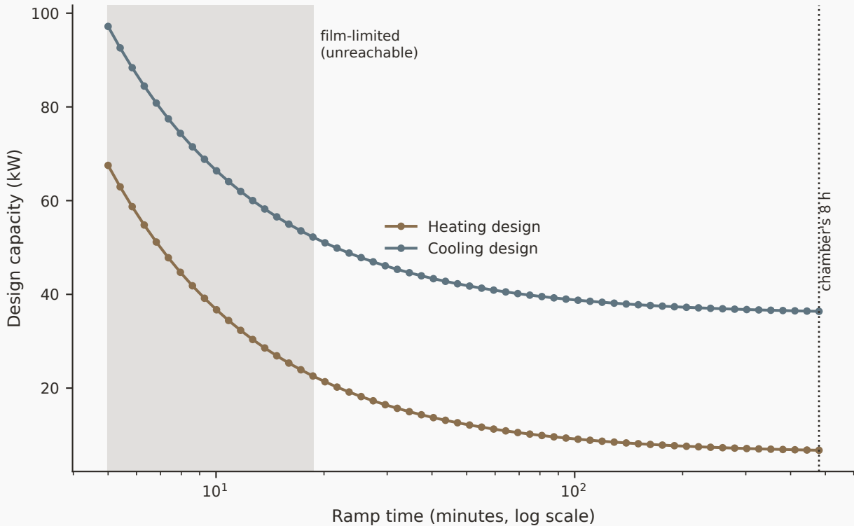
Module room, worst-case facade — design capacity vs ramp time
