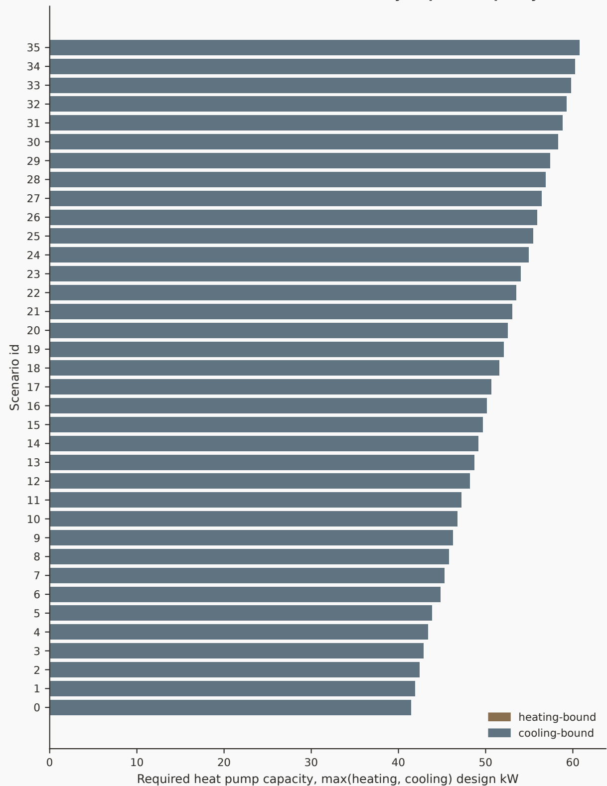
Climate chamber -- all 36 scenarios by required capacity
