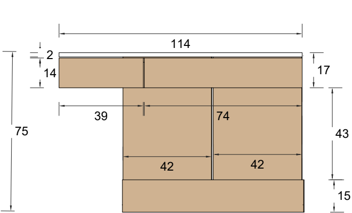
ELEVATION WORK TABLE
