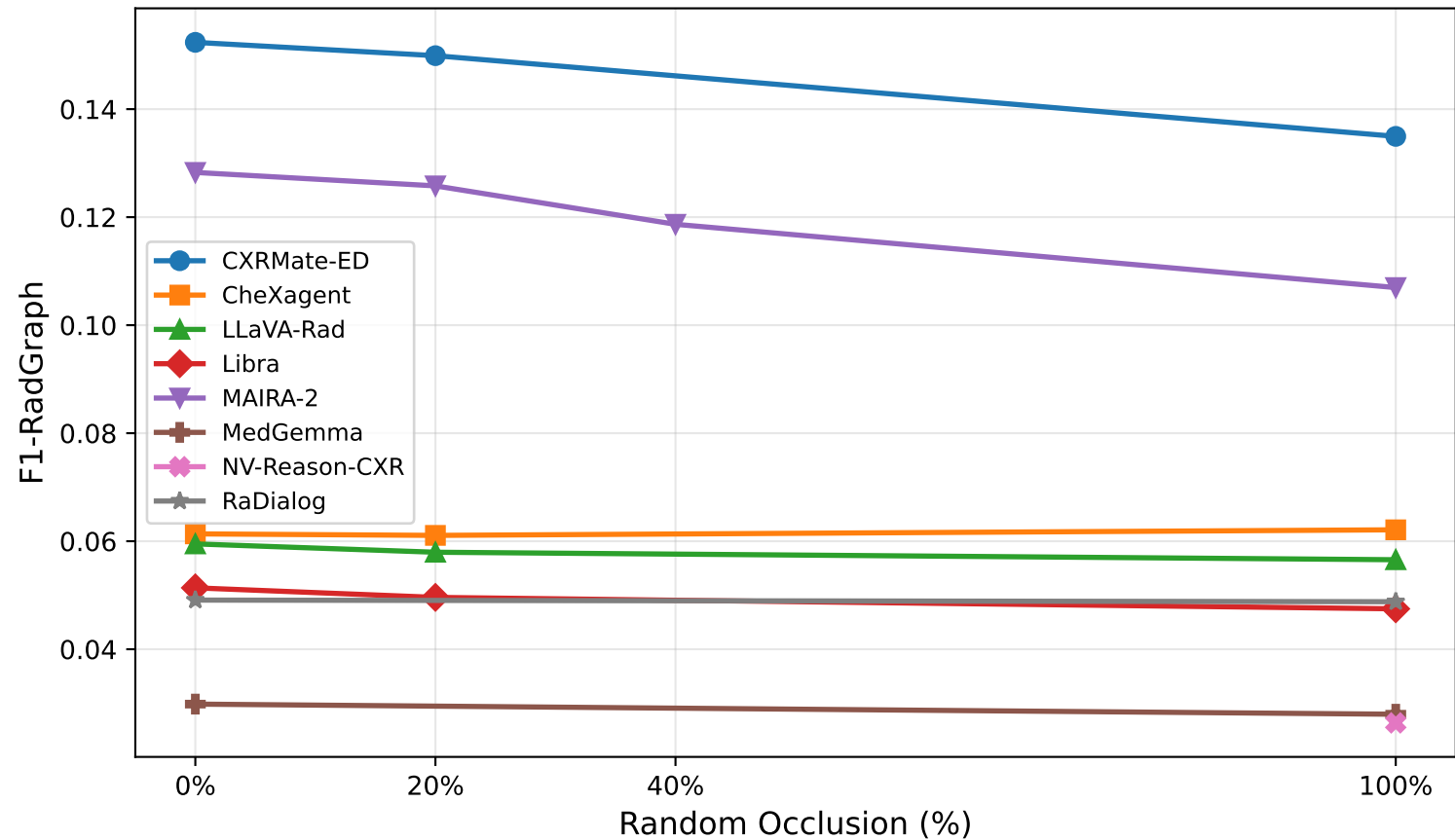
F1-RadGraph vs. Occlusion Level
