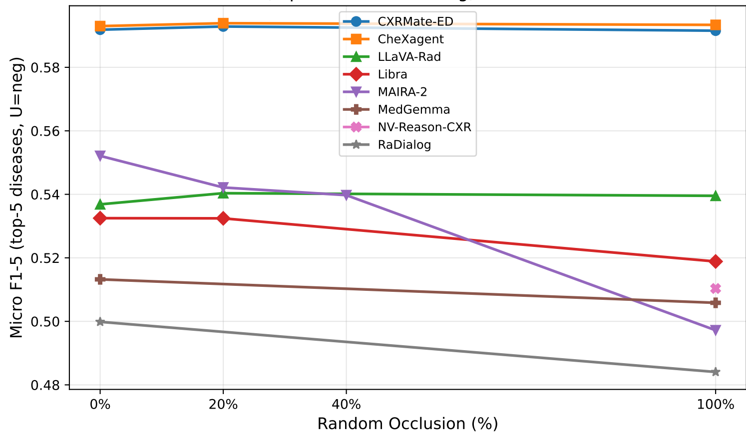
Micro F1-5 (top-5 diseases, U=neg) vs. Occlusion Level
