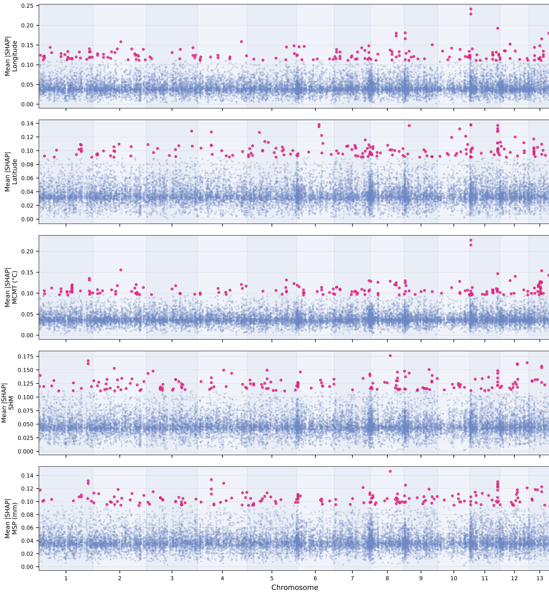
SHAP importance by real genomic position (Doug-fir, DFv5.29, all individuals)
