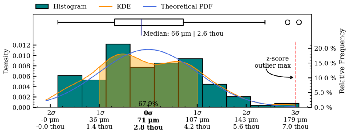
Figure 44: Coaxiality residual plots of interior_separate surface, HV001.
