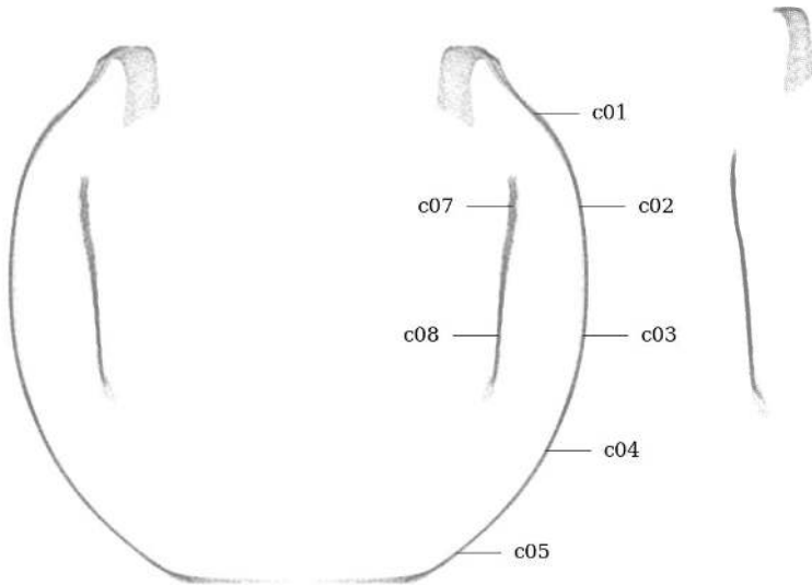
Figure 31: Circularity measurement sample locations, full mesh aligned to exterior surface
