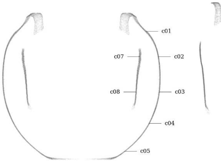
Figure 60: Circularity measurement sample locations, full mesh aligned to exterior surface
