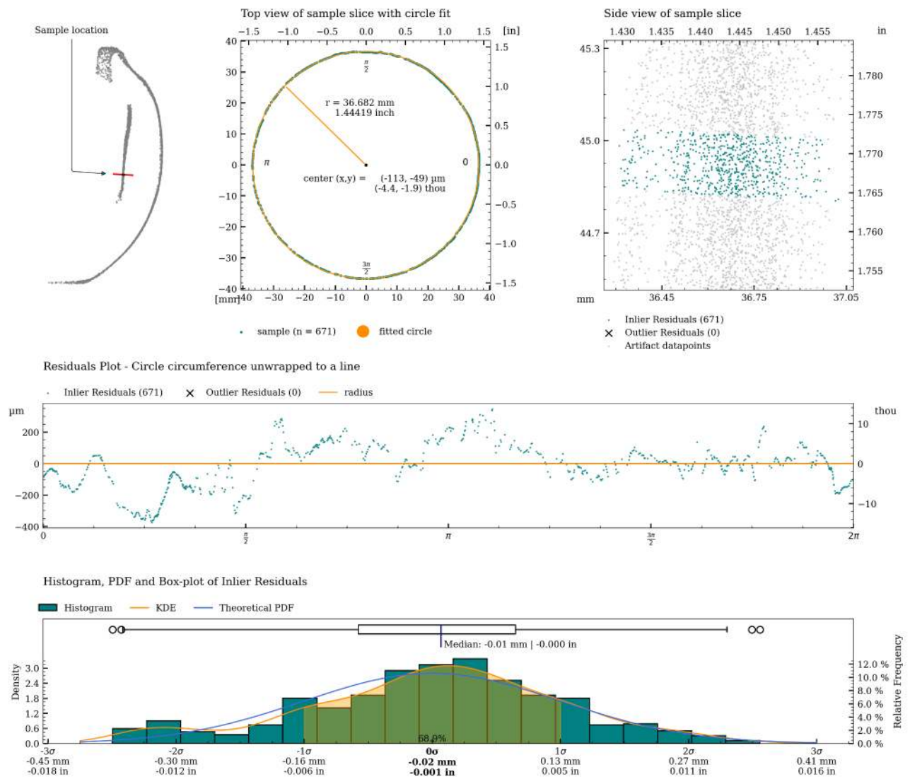
Figure 40: Detailed plot of concentricity measurement for c08.
