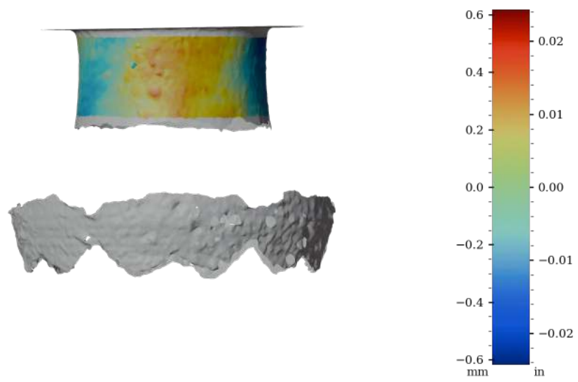
Figure 55: Surface variability heatmap of HV003, rotated 180°
