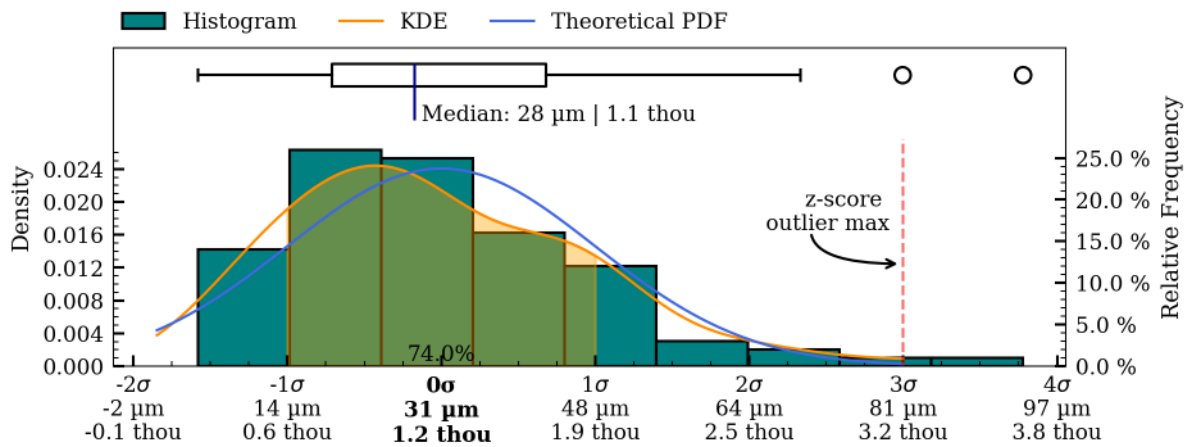
Figure 44: Coaxiality residual plots of interior_separate surface, HV003.
