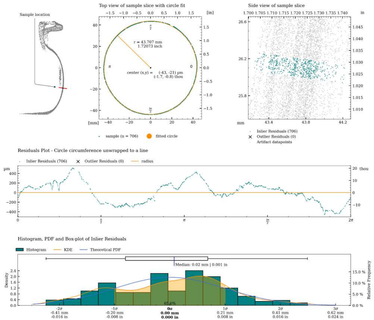
Figure 36: Detailed plot of concentricity measurement for c04.
