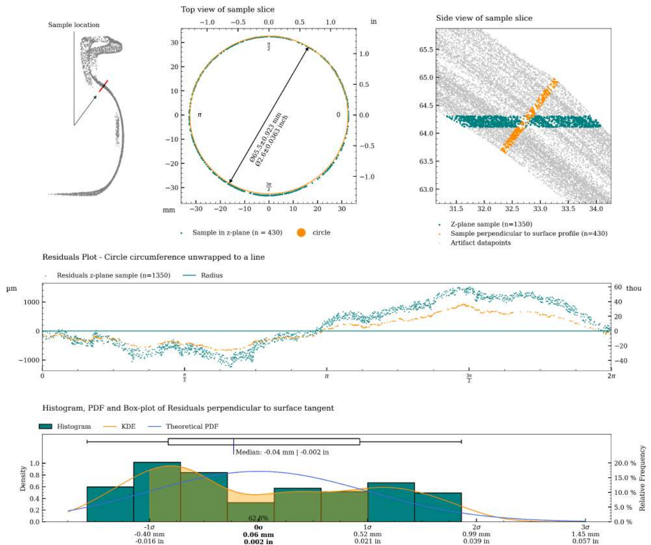
Figure 6: Charts with statistics for the measurement of c01.
