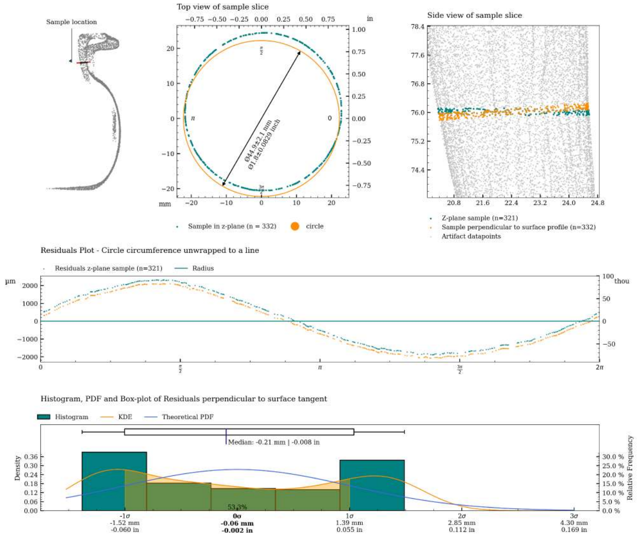
Figure 13: Charts with statistics for the measurement of c07.
