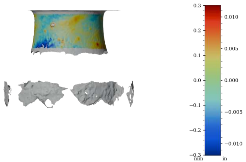
Figure 56: Surface variability heatmap of HV004, rotated 270°
