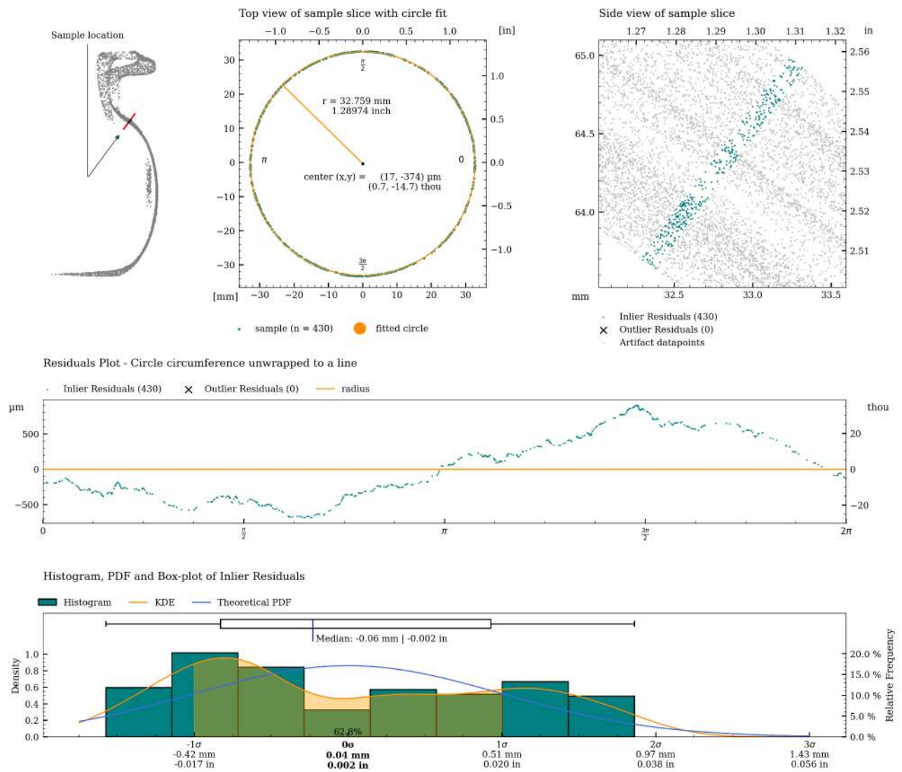
Figure 33: Detailed plot of concentricity measurement for c01.
