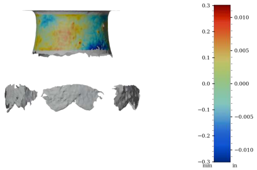
Figure 55: Surface variability heatmap of HV004, rotated 180°
