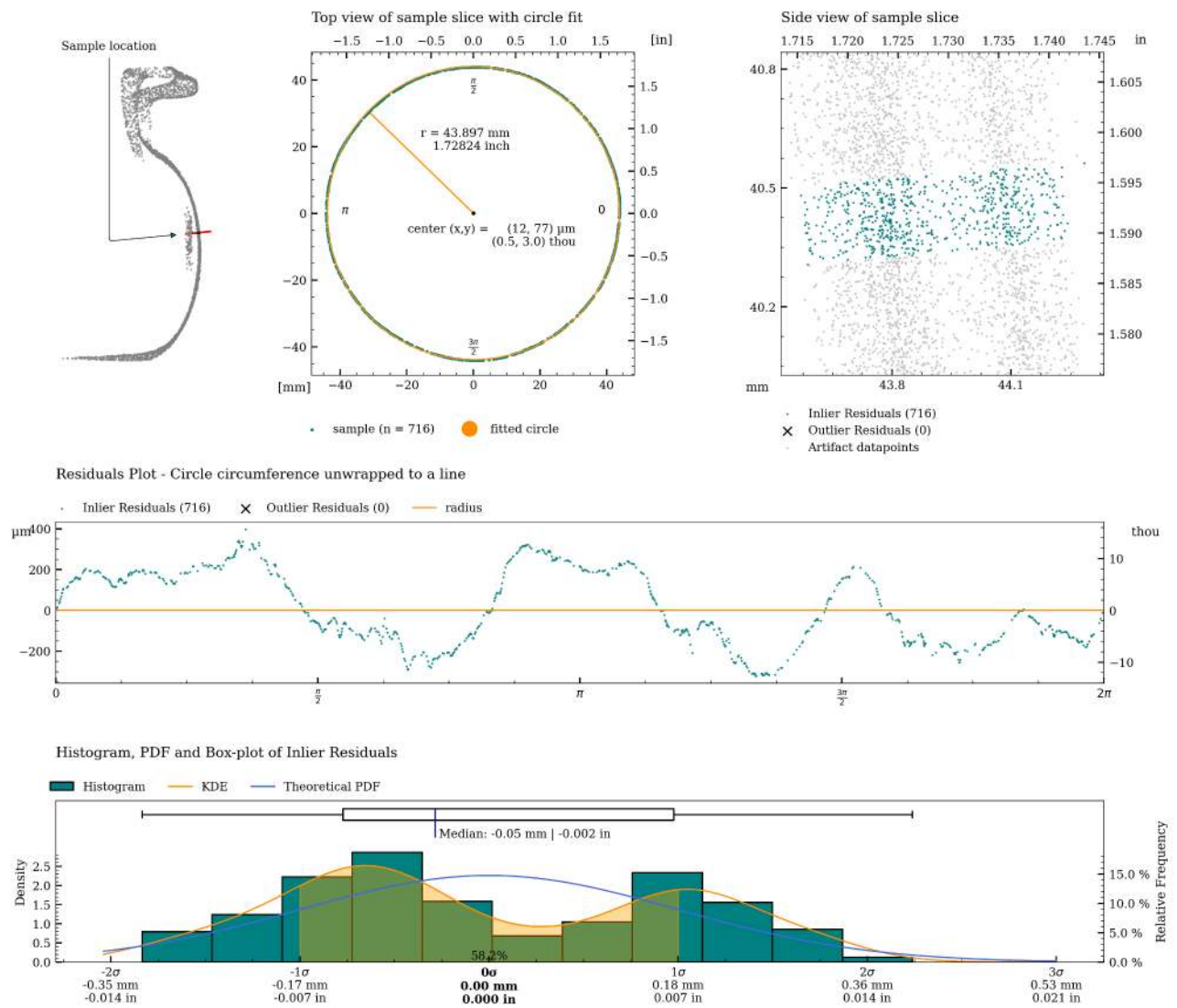
Figure 35: Detailed plot of concentricity measurement for c03.
