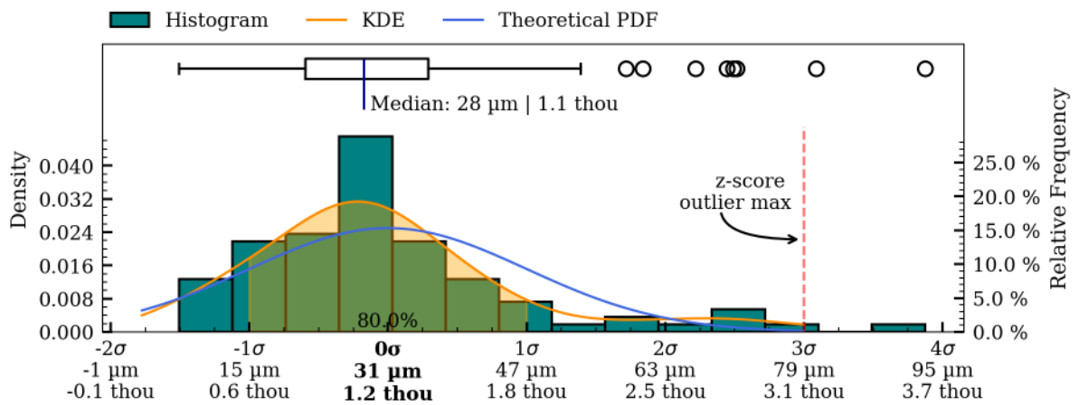
Figure 44: Coaxiality residual plots of interior_separate surface, HV005.
