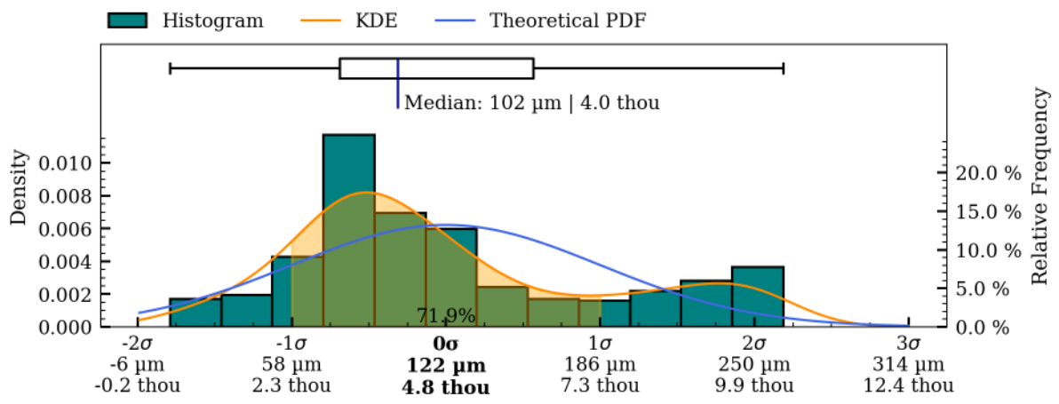
Figure 42: Coaxiality residual plots of exterior surface, HV005.
