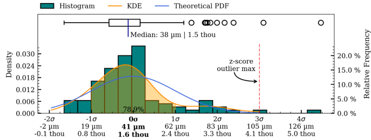
Figure 43: Coaxiality residual plots of interior surface, HV005.
