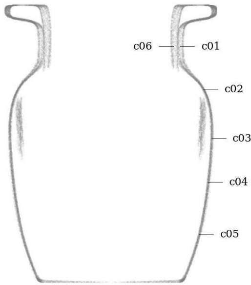
Figure 58: Circularity measurement sample locations, full mesh aligned to exterior surface
