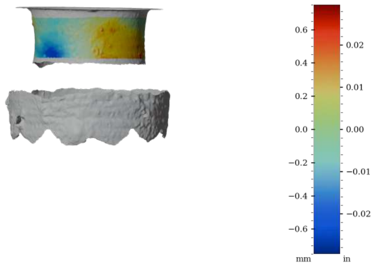
Figure 51: Surface variability heatmap of HV006, rotated 180°
