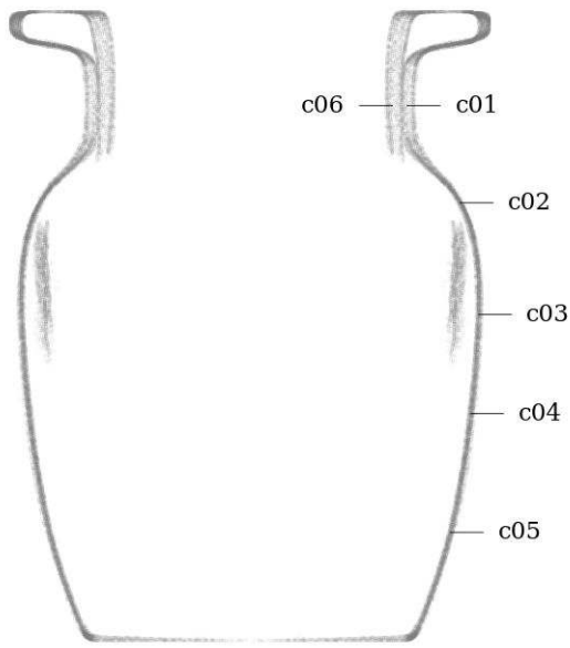
Figure 29: Circularity measurement sample locations, full mesh aligned to exterior surface
