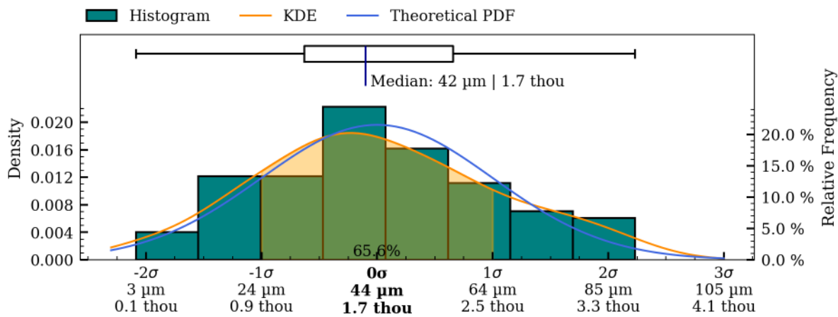
Figure 40: Coaxiality residual plots of interior_separate surface, HV006.
