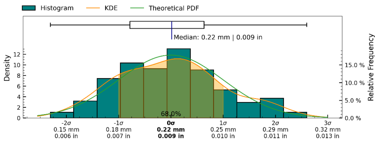
Figure 31: Root Mean Squared Deviation measurement distribution across measured slices of interior separately aligned surface
