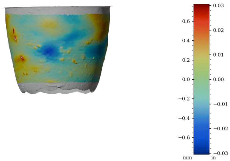
Figure 60: Surface variability heatmap of HV007, rotated 270°
