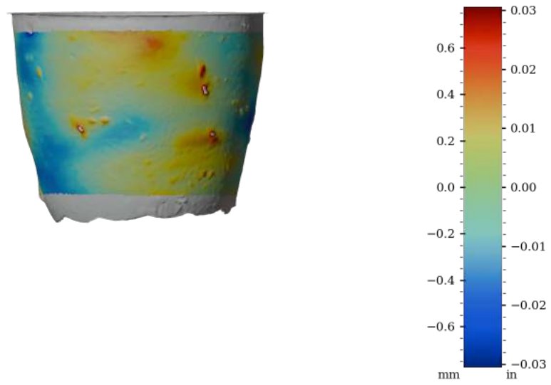
Figure 59: Surface variability heatmap of HV007, rotated 180°
