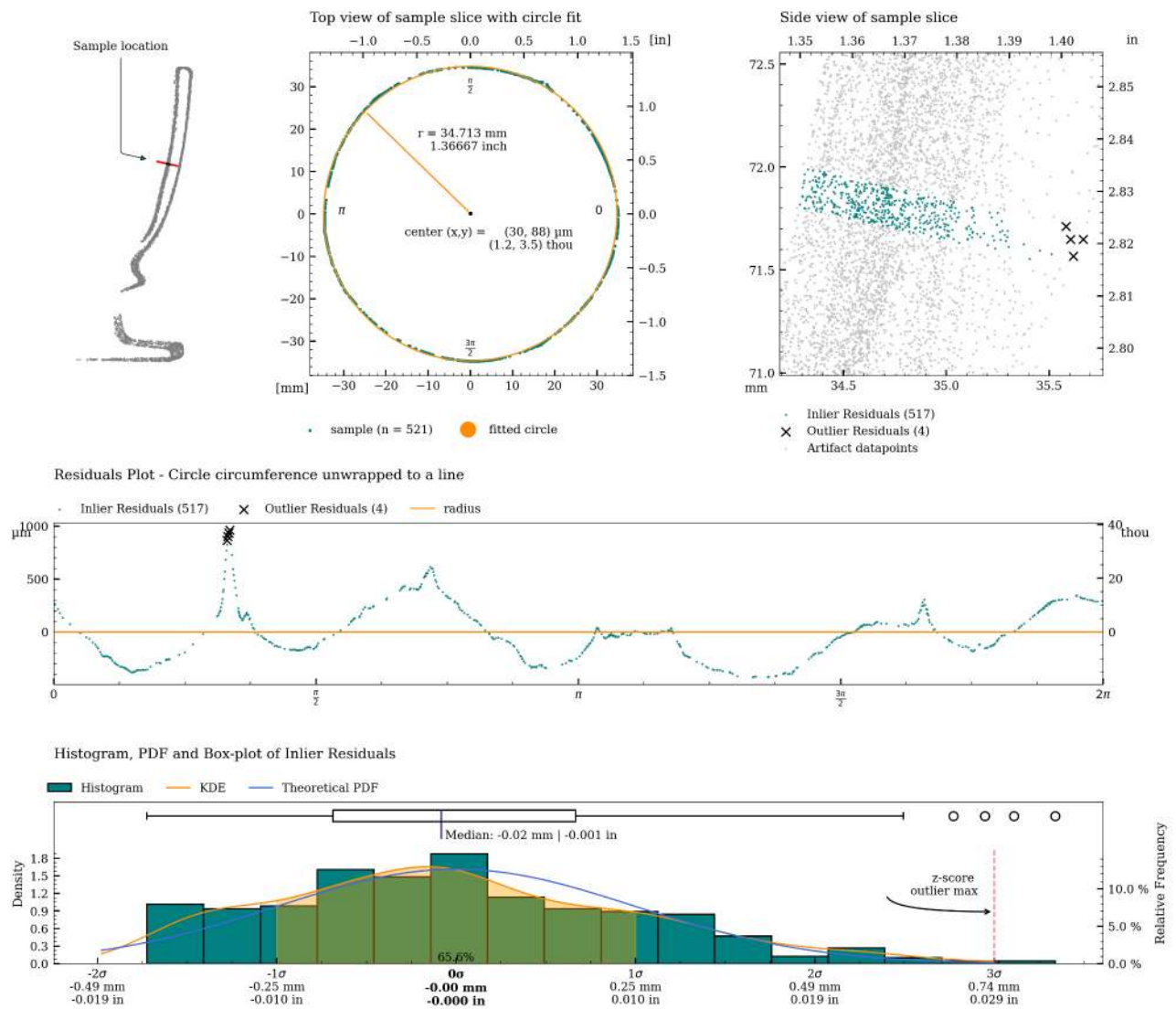
Figure 44: Detailed plot of concentricity measurement for c08.
