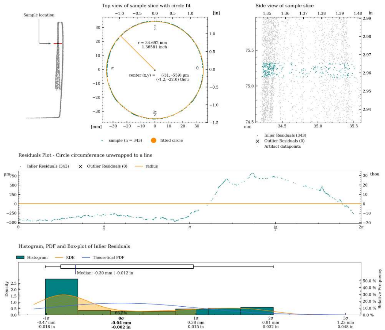
Figure 39: Detailed plot of concentricity measurement for c07.
