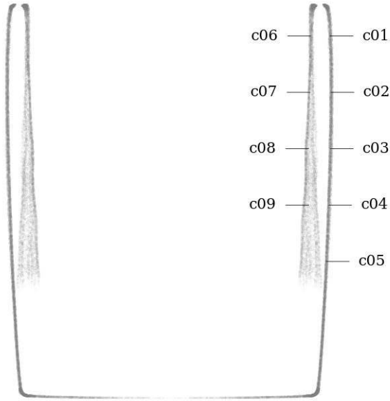
Figure 62: Circularity measurement sample locations, full mesh aligned to exterior surface
