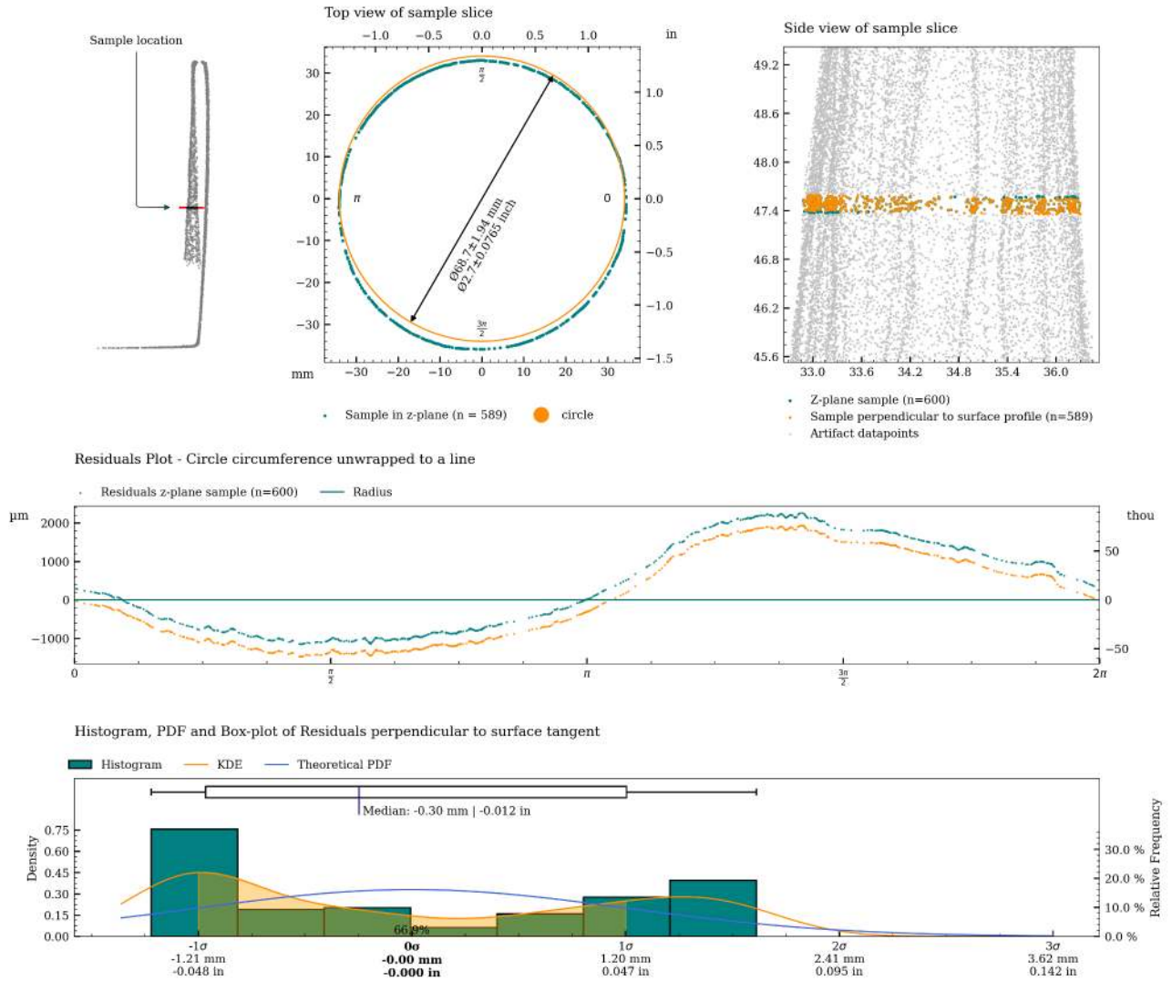
Figure 14: Charts with statistics for the measurement of c09.
