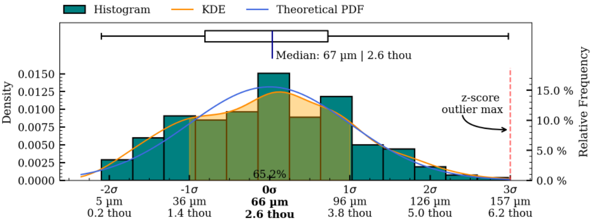
Figure 42: Coaxiality residual plots of exterior surface, HV008.
