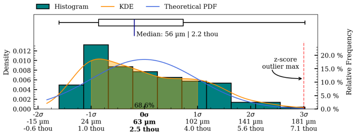
Figure 44: Coaxiality residual plots of interior_separate surface, HV008.
