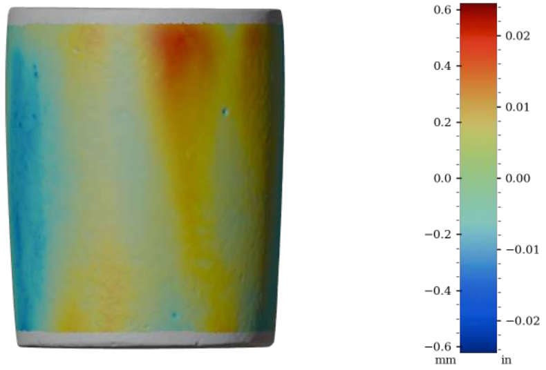
Figure 47: Surface variability heatmap of HV008, rotated 180°
