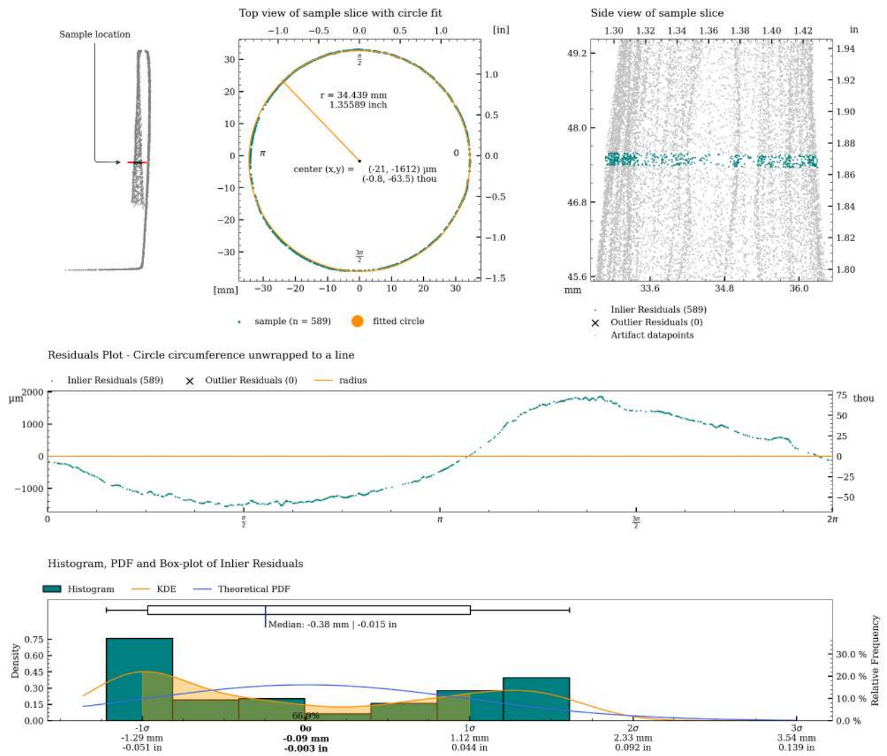
Figure 41: Detailed plot of concentricity measurement for c09.
