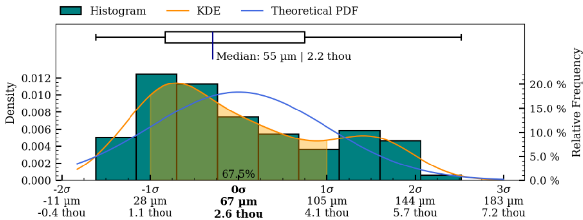
Figure 43: Coaxiality residual plots of interior surface, HV008.
