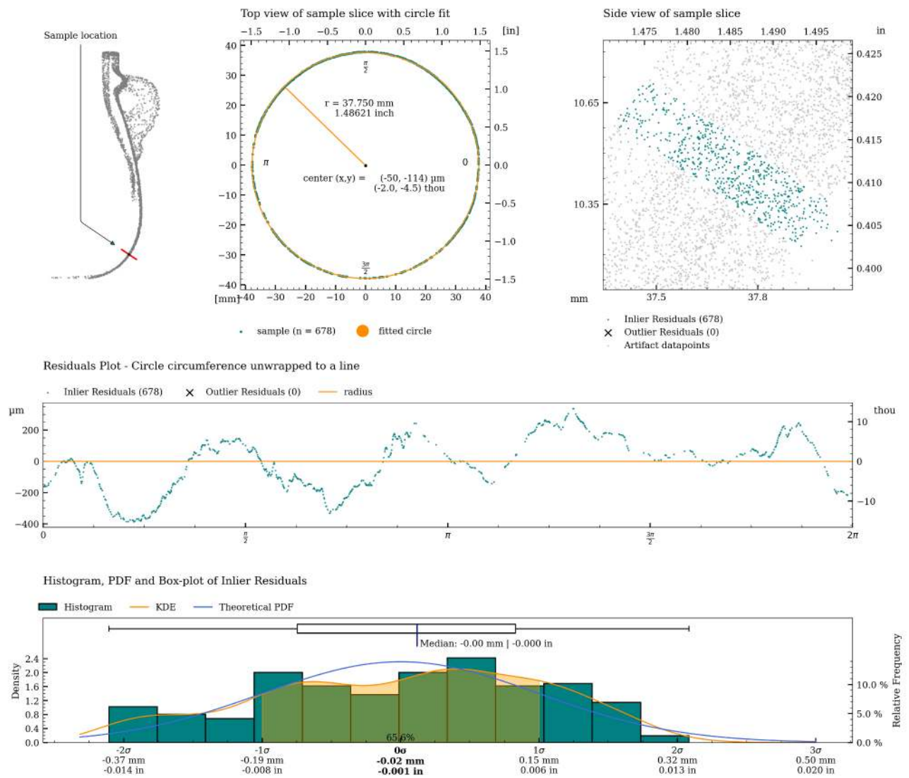
Figure 35: Detailed plot of concentricity measurement for c05.
