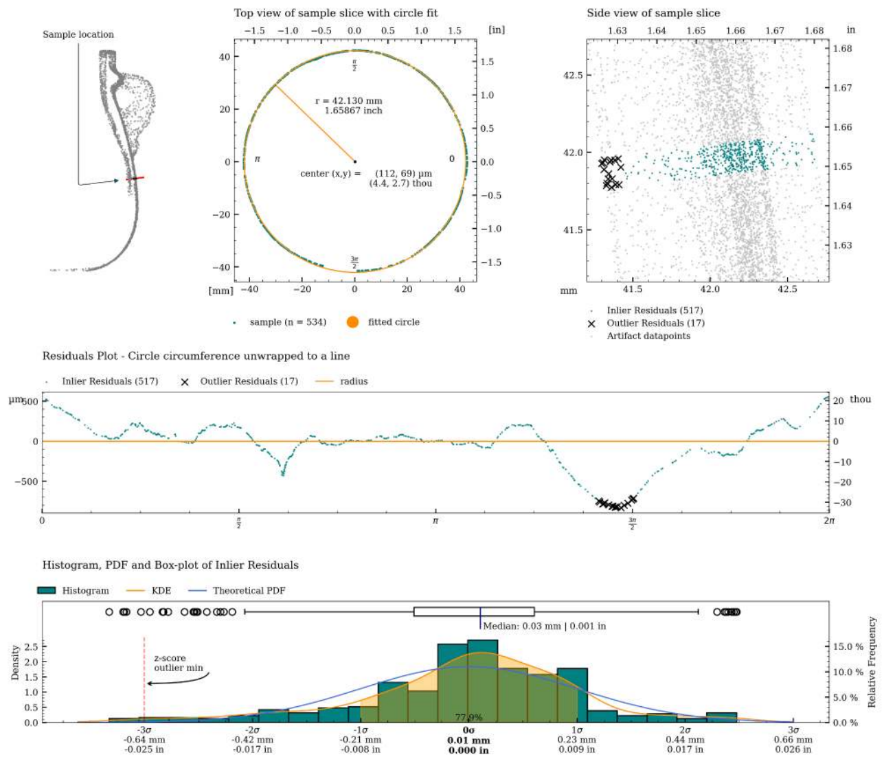
Figure 33: Detailed plot of concentricity measurement for c03.
