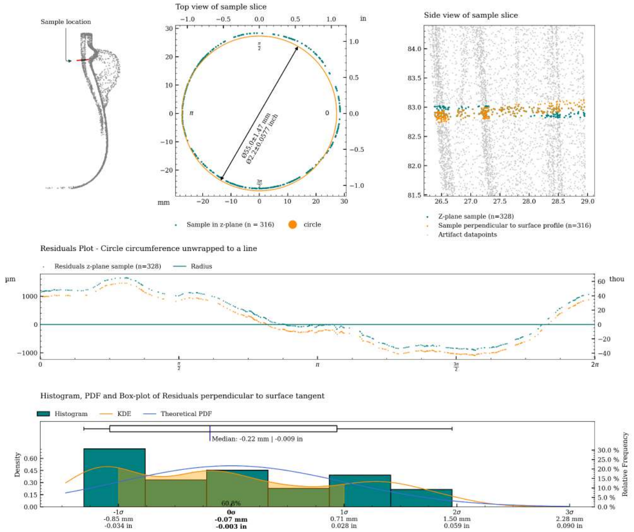
Figure 12: Charts with statistics for the measurement of c07.
