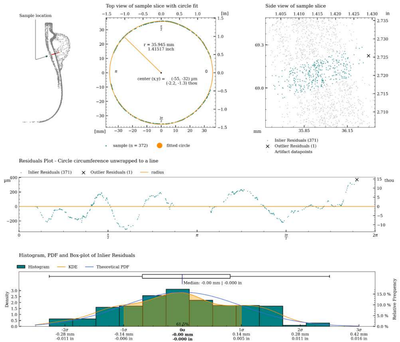
Figure 31: Detailed plot of concentricity measurement for c01.
