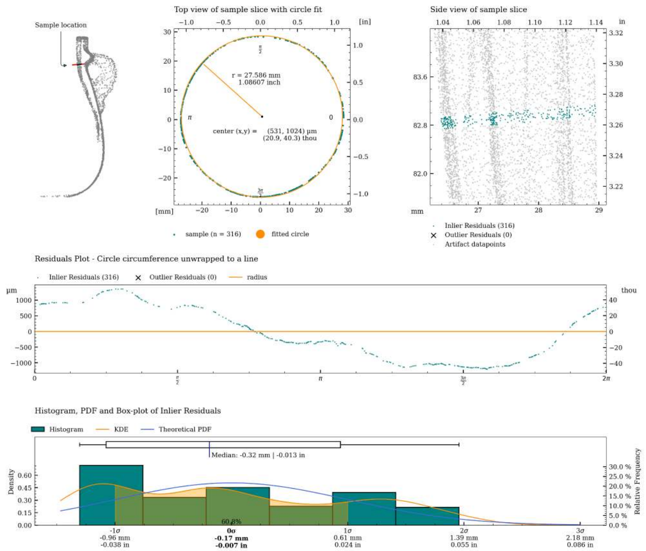
Figure 37: Detailed plot of concentricity measurement for c07.
