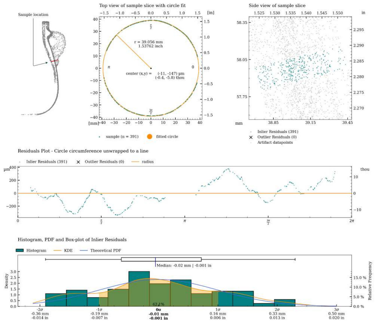
Figure 32: Detailed plot of concentricity measurement for c02.
