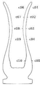
Figure 74: Circularity measurement sample locations, full mesh aligned to exterior surface
