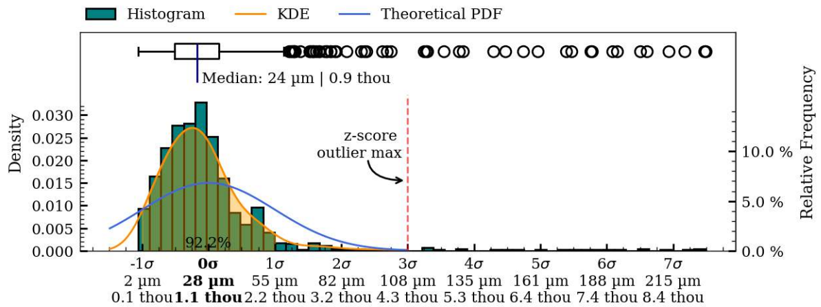
Figure 54: Coaxiality residual plots of exterior surface, IV001.
