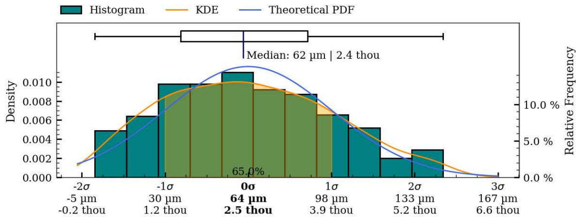
Figure 56: Coaxiality residual plots of interior_separate surface, IV002.
