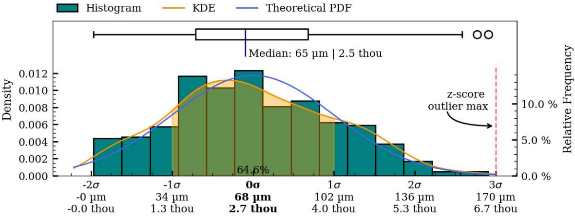
Figure 55: Coaxiality residual plots of interior surface, IV002.
