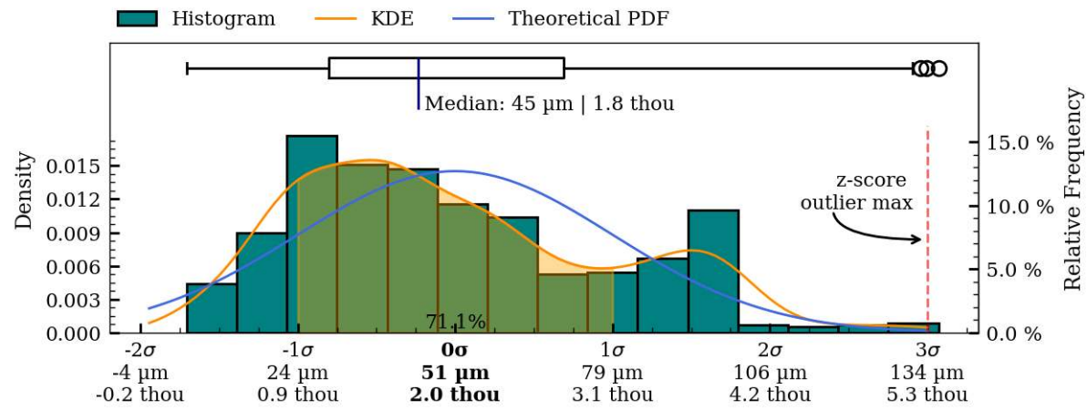
Figure 54: Coaxiality residual plots of exterior surface, IV002.
