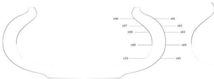
Figure 74: Circularity measurement sample locations, full mesh aligned to exterior surface
