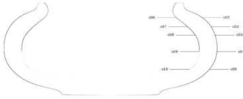
Figure 72: Circularity measurement sample locations, full mesh aligned to exterior surface
