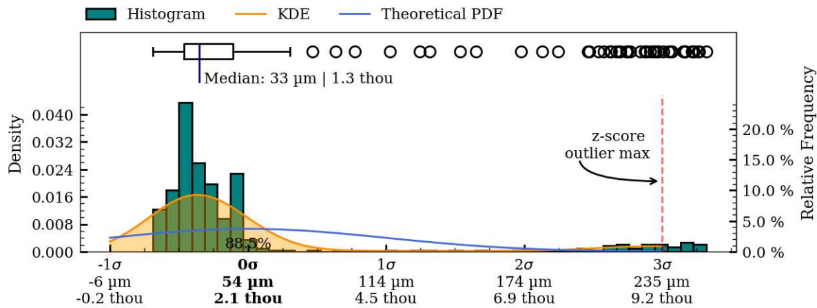
Figure 56: Coaxiality residual plots of interior_separate surface, IV003.
