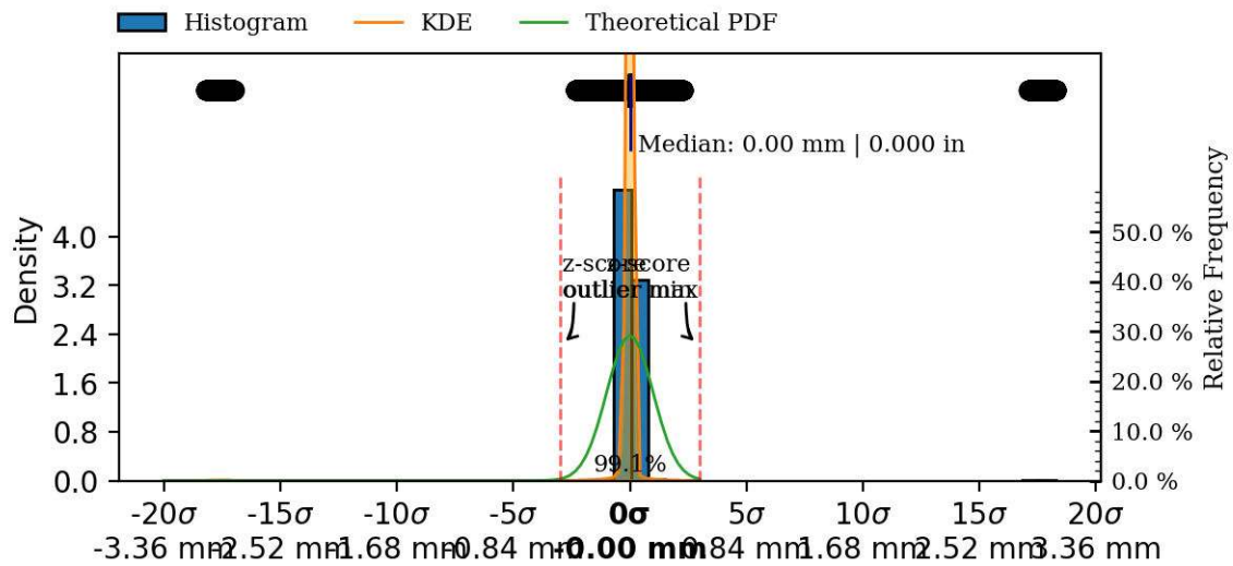
Figure 69: Exterior surface variability boxplot, kds and histogram.
