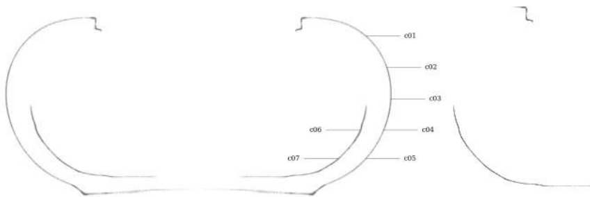
Figure 31: Circularity measurement sample locations, full mesh aligned to exterior surface
