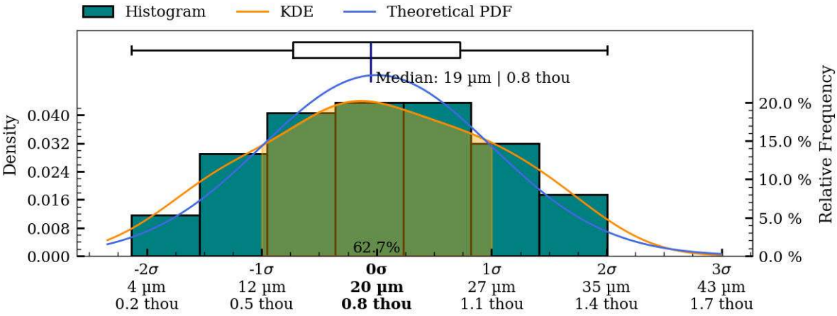
Figure 43: Coaxiality residual plots of interior surface, IV005.
