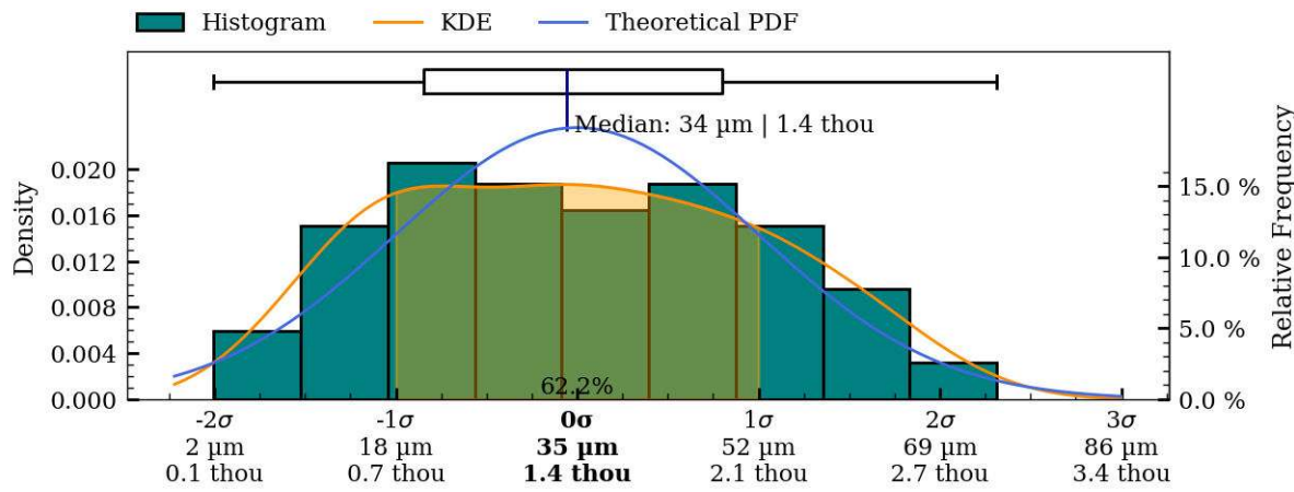
Figure 42: Coaxiality residual plots of exterior surface, IV005.
