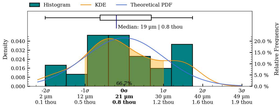
Figure 44: Coaxiality residual plots of interior_separate surface, IV005.
