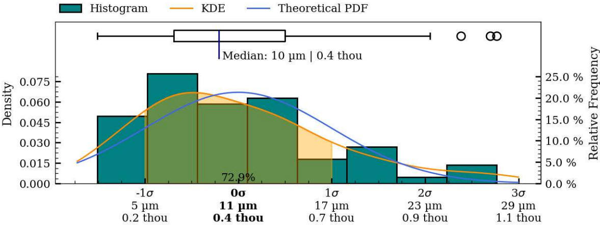
Figure 43: Coaxiality residual plots of interior surface, IV006.
