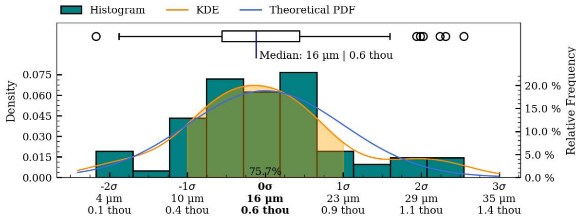
Figure 44: Coaxiality residual plots of interior_separate surface, IV006.
