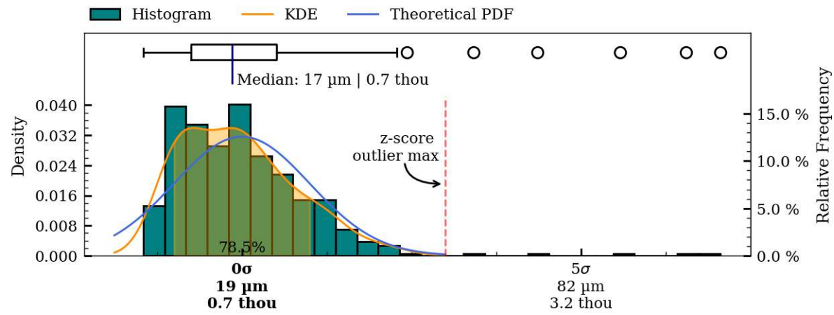
Figure 42: Coaxiality residual plots of exterior surface, IV006.
