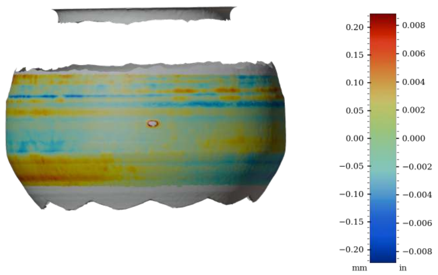
Figure 55: Surface variability heatmap of IV007, rotated 180°
