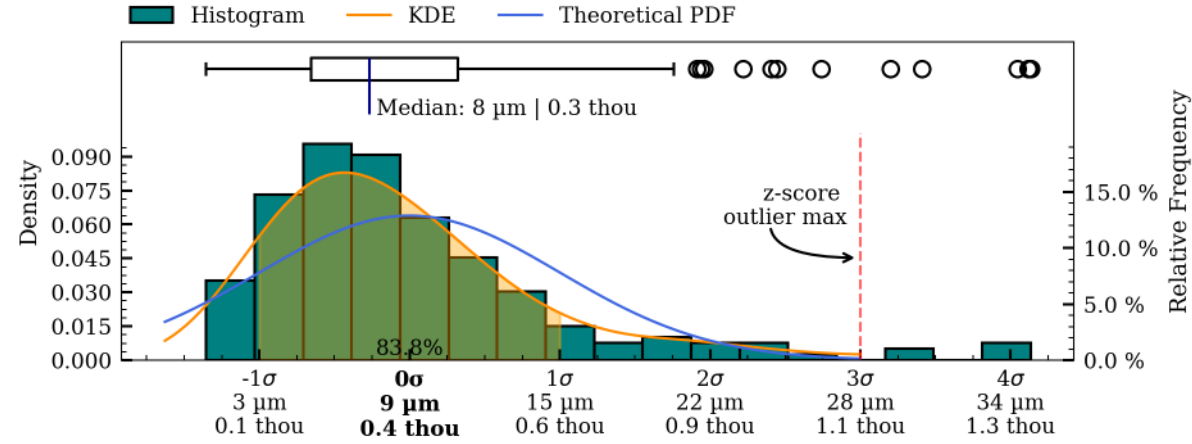
Figure 48: Coaxiality residual plots of interior_separate surface, IV007.
