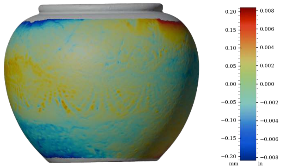
Figure 51: Surface variability heatmap of IV007, rotated 180°
