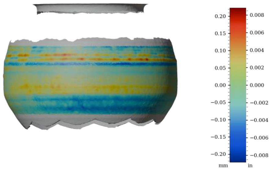
Figure 56: Surface variability heatmap of IV007, rotated 270°
