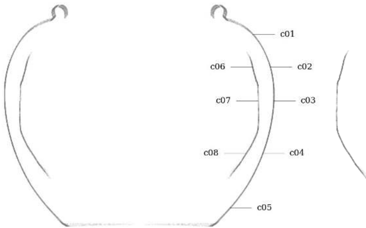
Figure 64: Circularity measurement sample locations, full mesh aligned to exterior surface
