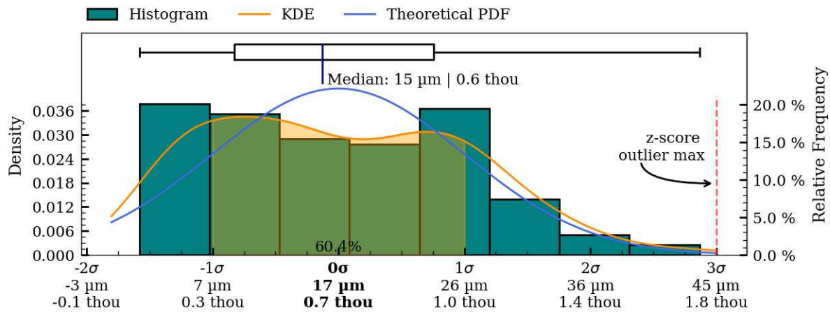
Figure 44: Coaxiality residual plots of interior_separate surface, IV008.
