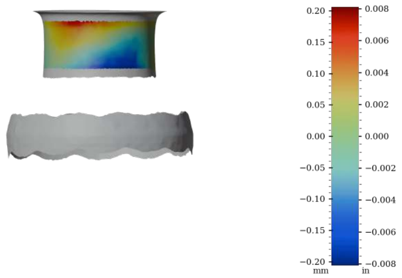
Figure 55: Surface variability heatmap of IV009, rotated 180°
