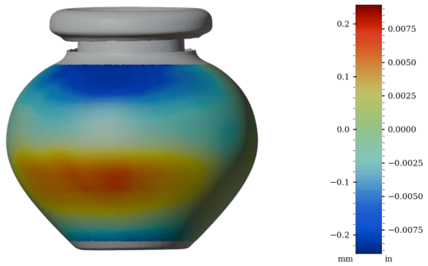
Figure 47: Surface variability heatmap of IV009, rotated 180°
