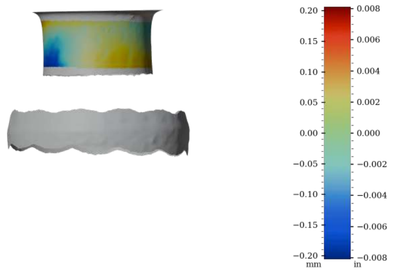
Figure 56: Surface variability heatmap of IV009, rotated 270°
