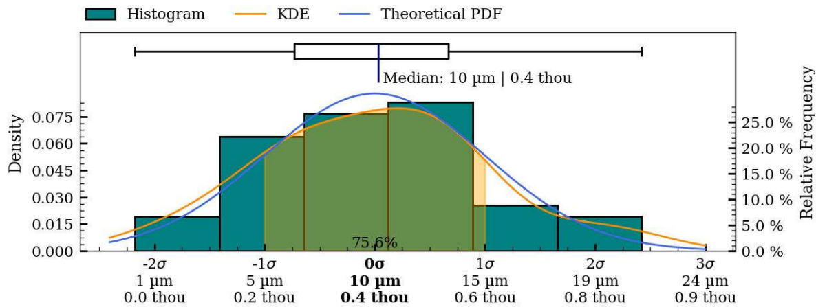
Figure 44: Coaxiality residual plots of interior_separate surface, IV009.
