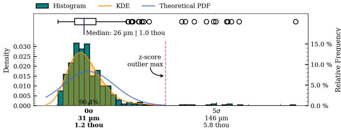
Figure 38: Coaxiality residual plots of exterior surface, IV012.
