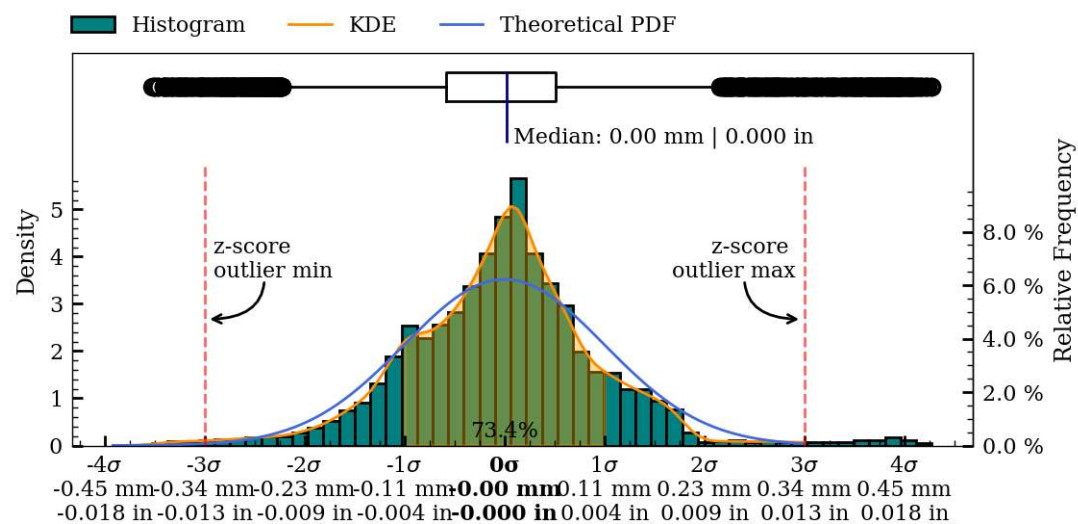
Figure 55: Interior separately aligned surface variability boxplot, kds and histogram.
