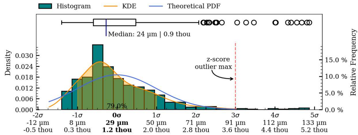
Figure 38: Coaxiality residual plots of exterior surface, IV014.
