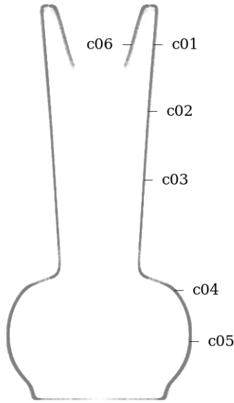
Figure 4: Circularity measurement sample locations, full mesh aligned with exterior surface
