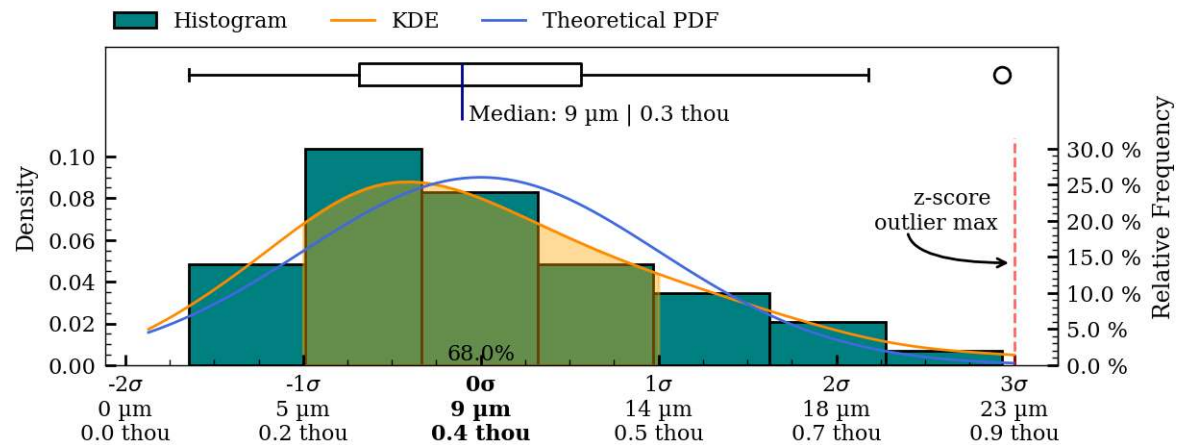
Figure 39: Coaxiality residual plots of interior surface, IV014.
