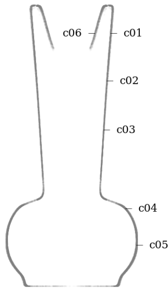
Figure 58: Circularity measurement sample locations, full mesh aligned to exterior surface
