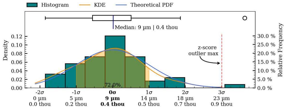
Figure 40: Coaxiality residual plots of interior_separate surface, IV014.
