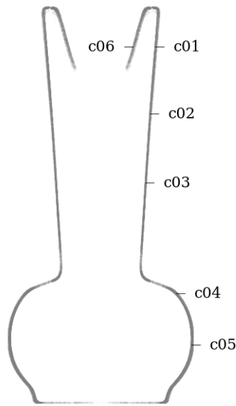
Figure 29: Circularity measurement sample locations, full mesh aligned to exterior surface
