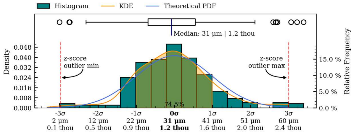
Figure 48: Coaxiality residual plots of interior_separate surface, IV018.
