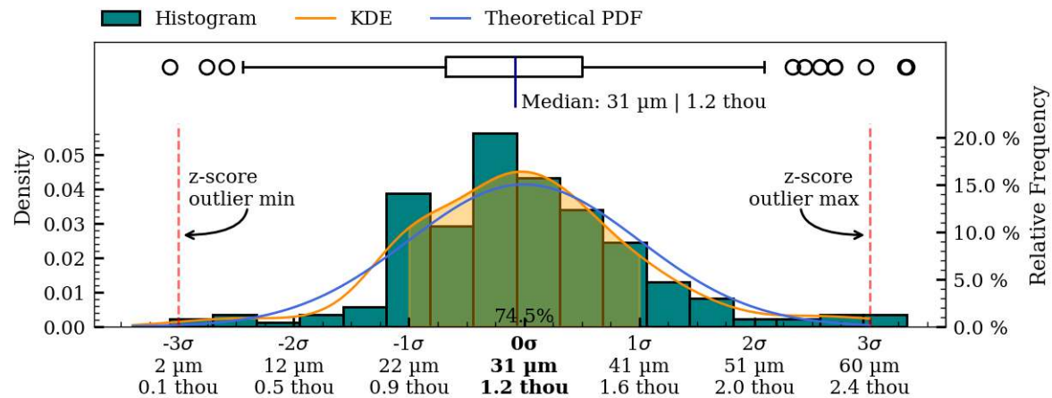
Figure 47: Coaxiality residual plots of interior surface, IV018.
