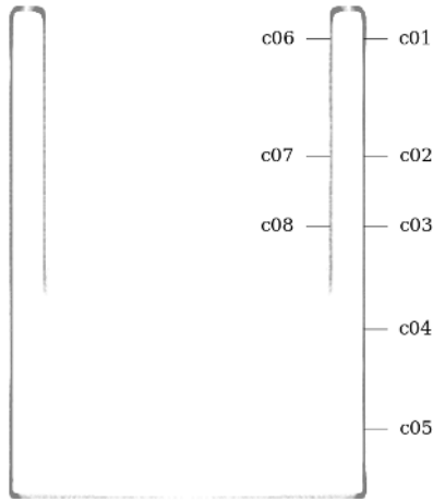
Figure 64: Circularity measurement sample locations, full mesh aligned to exterior surface
