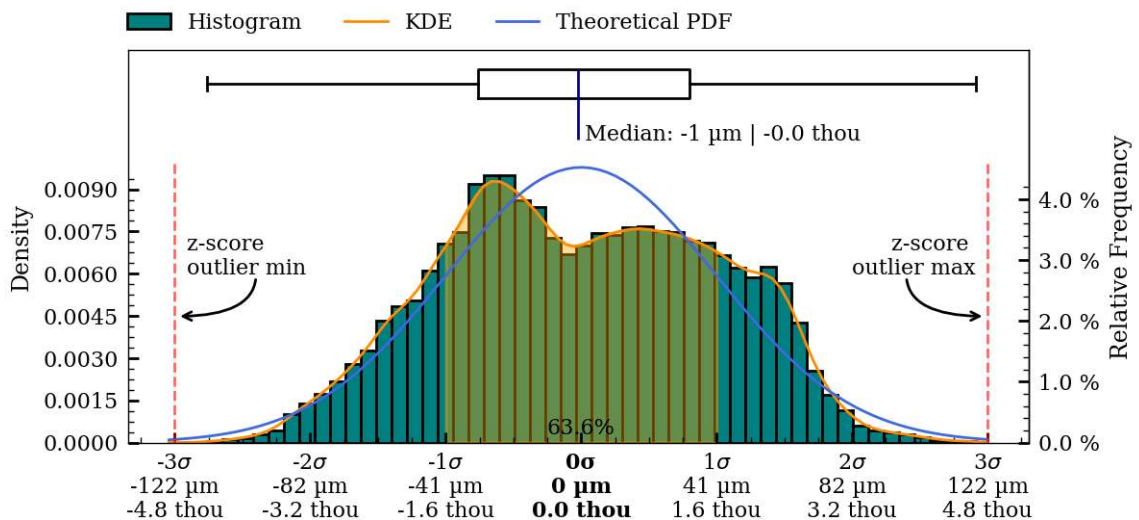
Figure 62: Interior surface variability boxplot, kds and histogram.
