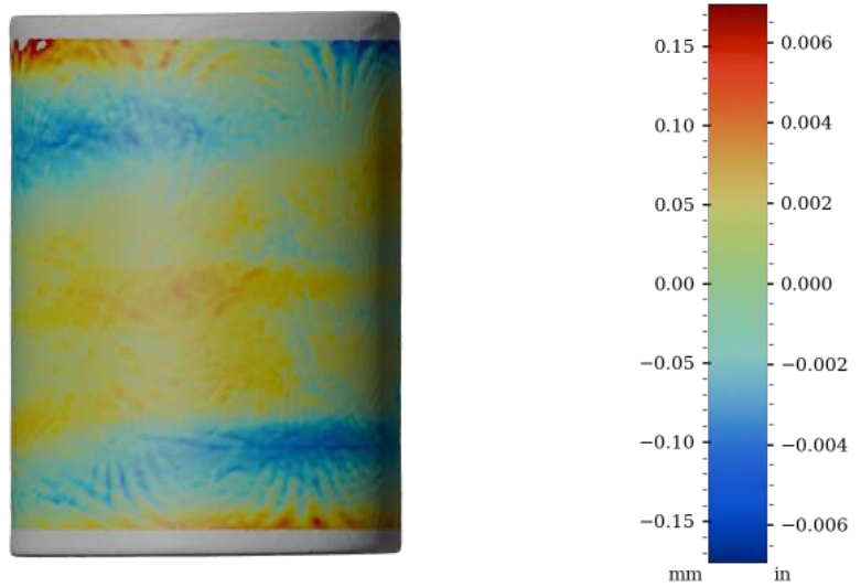
Figure 52: Surface variability heatmap of IV018, rotated 270°
