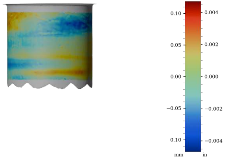
Figure 55: Surface variability heatmap of IV018, rotated 180°
