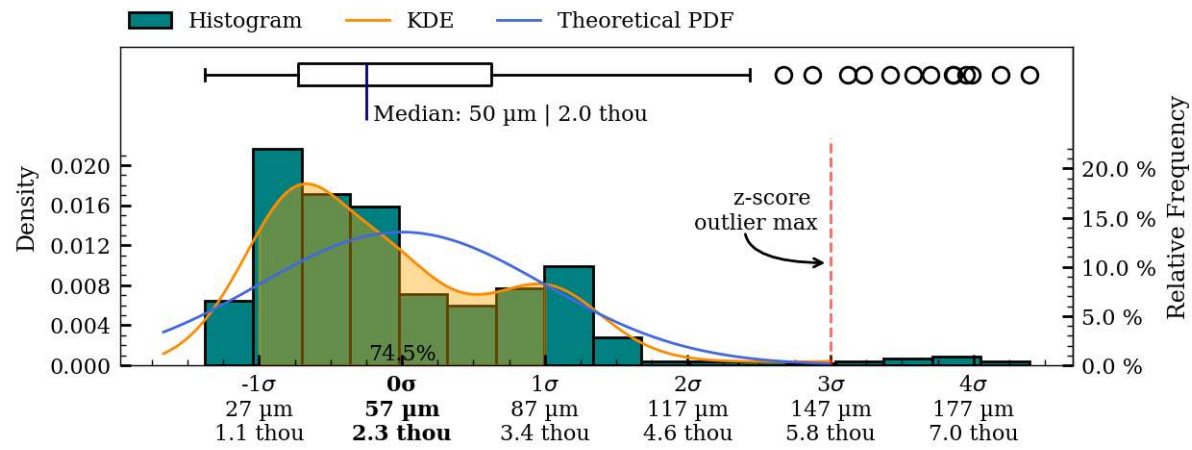
Figure 46: Coaxiality residual plots of exterior surface, IV018.
