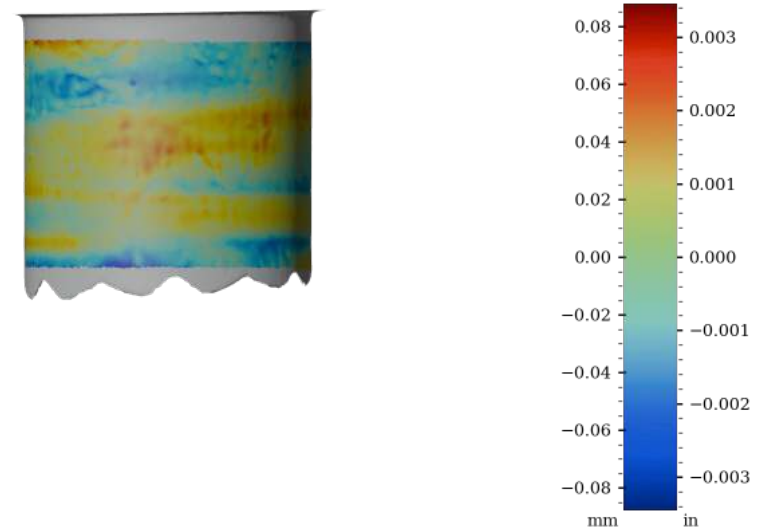
Figure 60: Surface variability heatmap of IV018, rotated 270°
