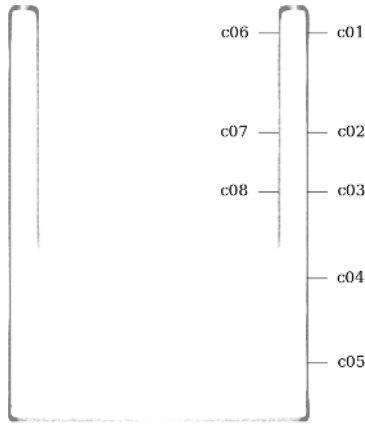
Figure 33: Circularity measurement sample locations, full mesh aligned to exterior surface
