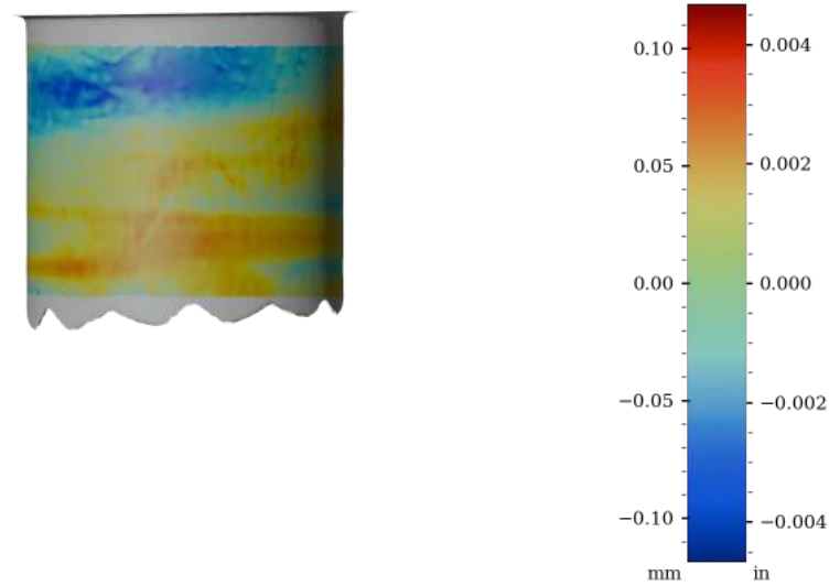
Figure 56: Surface variability heatmap of IV018, rotated 270°
