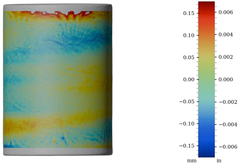
Figure 51: Surface variability heatmap of IV018, rotated 180°
