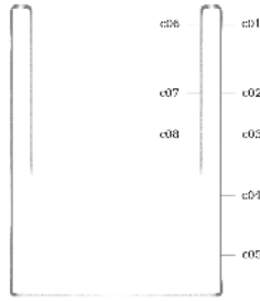
Figure 80: Circularity measurement sample locations, full mesh aligned to exterior surface
