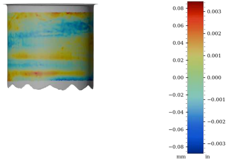
Figure 59: Surface variability heatmap of IV018, rotated 180°
