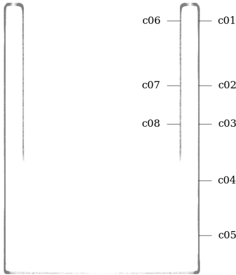
Figure 66: Circularity measurement sample locations, full mesh aligned to exterior surface
