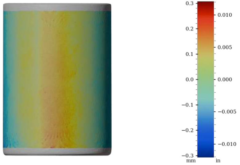
Figure 51: Surface variability heatmap of IV019, rotated 180°
