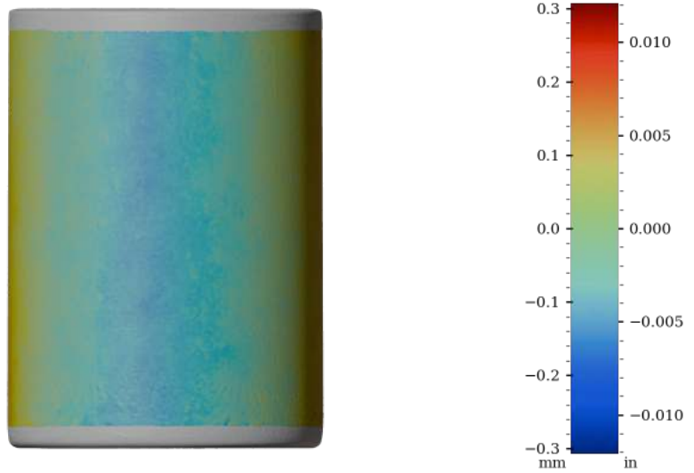
Figure 52: Surface variability heatmap of IV019, rotated 270°
