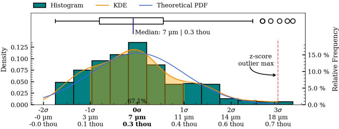
Figure 47: Coaxiality residual plots of interior surface, IV019.
