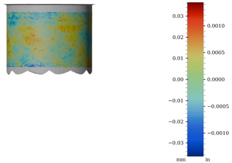
Figure 60: Surface variability heatmap of IV019, rotated 270°
