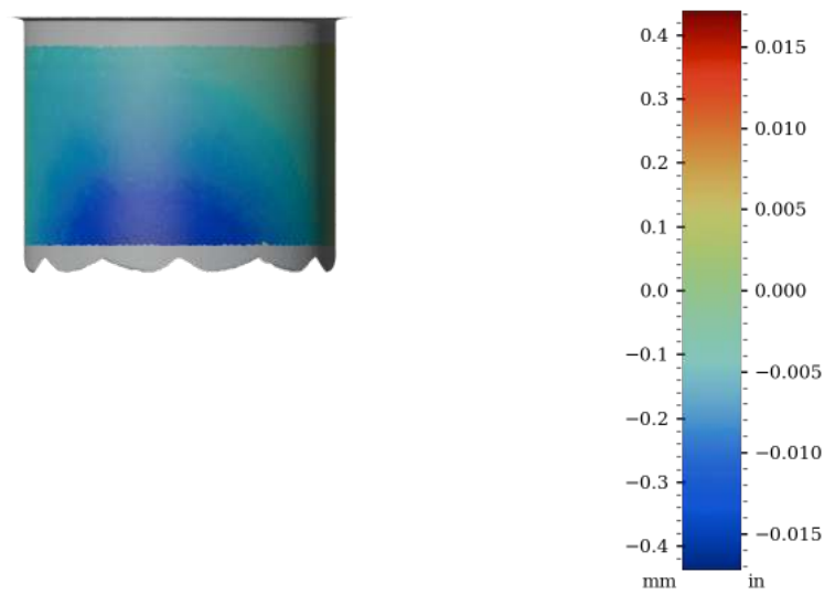
Figure 56: Surface variability heatmap of IV019, rotated 270°
