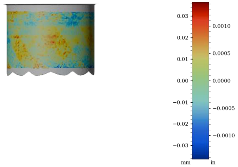
Figure 59: Surface variability heatmap of IV019, rotated 180°
