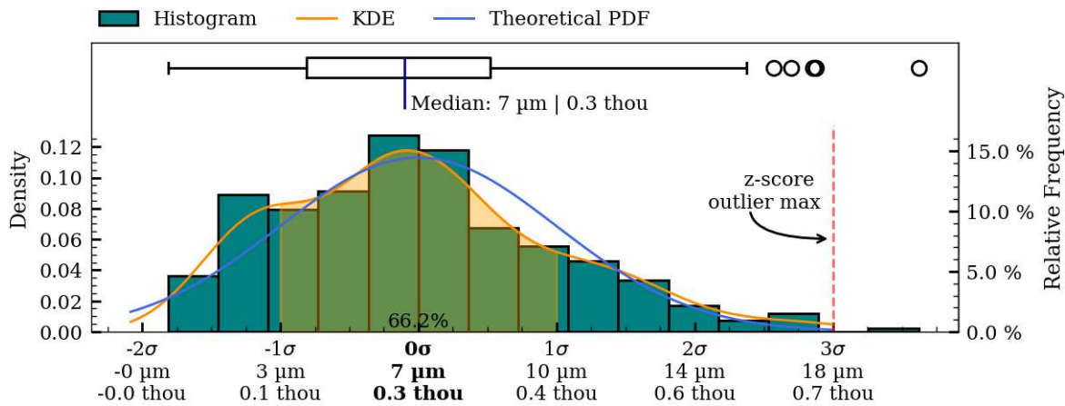
Figure 48: Coaxiality residual plots of interior_separate surface, IV019.
