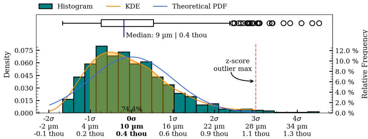
Figure 46: Coaxiality residual plots of exterior surface, IV019.
