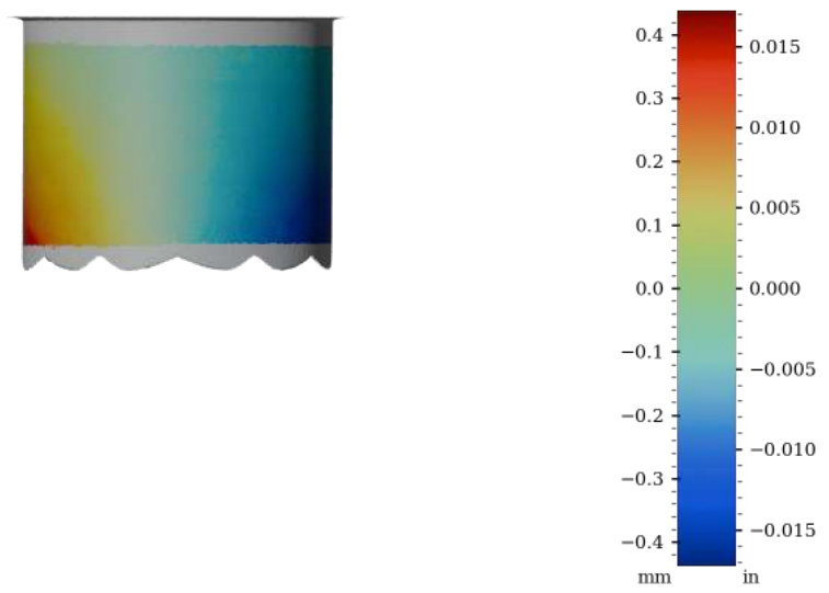
Figure 55: Surface variability heatmap of IV019, rotated 180°
