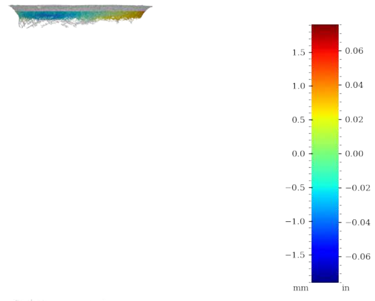
Figure 48: Surface variability heatmap of MV001, rotated 270°
