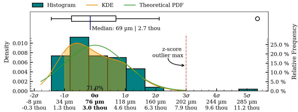
Figure 39: Coaxiality residual plots of interior surface, MV001.
