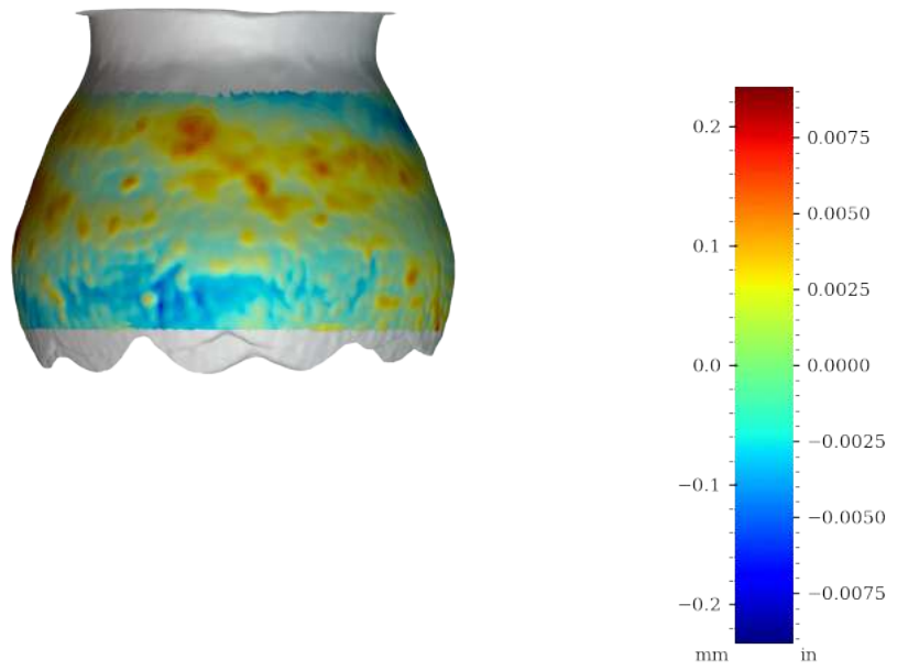
Figure 59: Surface variability heatmap of MV003b, rotated 180°
