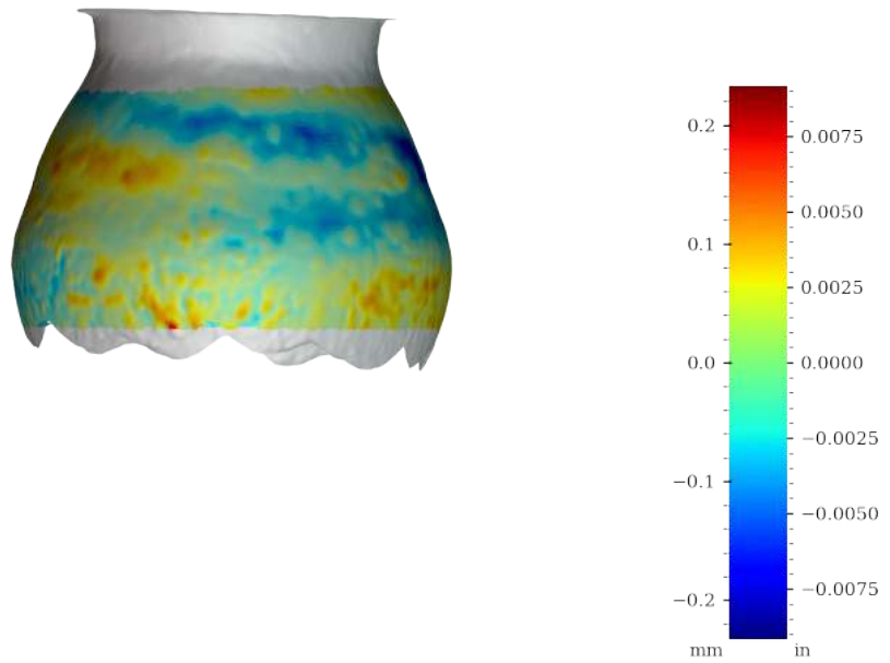
Figure 60: Surface variability heatmap of MV003b, rotated 270°
