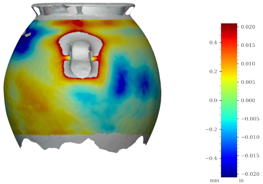
Figure 52: Surface variability heatmap of MV003b, rotated 270°
