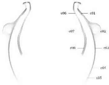
Figure 80: Circularity measurement sample locations, full mesh aligned to exterior surface
