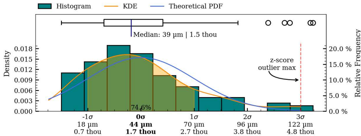
Figure 48: Coaxiality residual plots of interior_separate surface, MV003b.
