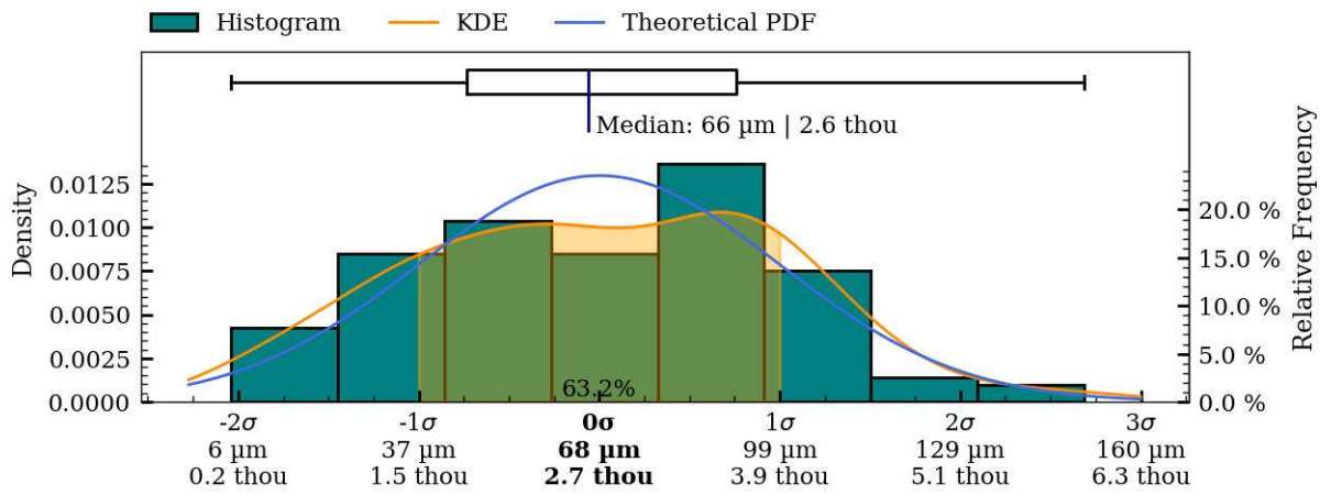
Figure 47: Coaxiality residual plots of interior surface, MV003b.
