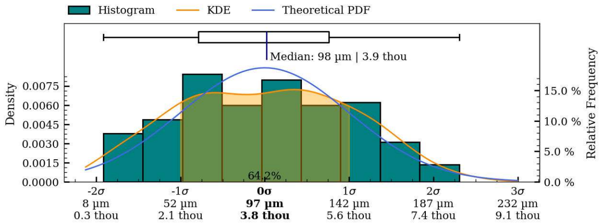
Figure 46: Coaxiality residual plots of exterior surface, MV003b.
