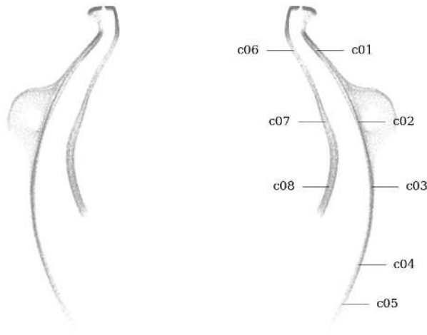
Figure 64: Circularity measurement sample locations, full mesh aligned to exterior surface
