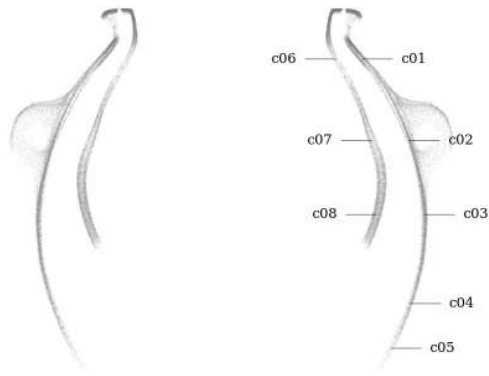
Figure 82: Circularity measurement sample locations, full mesh aligned to exterior surface
