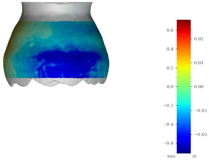
Figure 55: Surface variability heatmap of MV003b, rotated 180°
