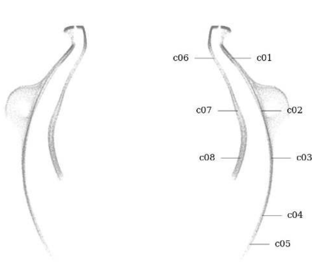
Figure 66: Circularity measurement sample locations, full mesh aligned to exterior surface
