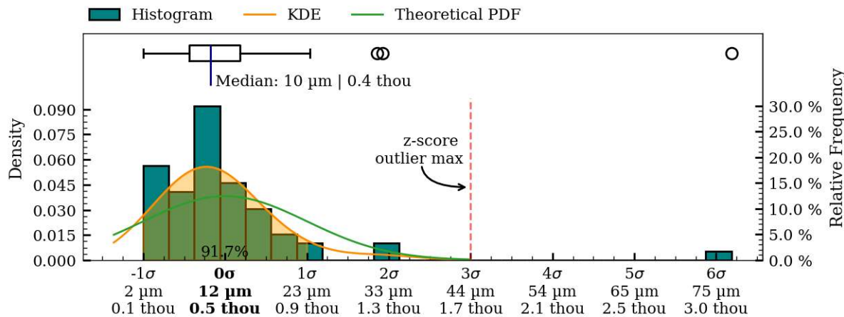
Figure 39: Coaxiality residual plots of interior surface, MV004.
