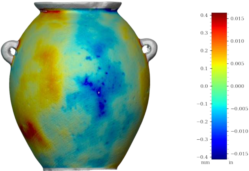
Figure 41: Surface variability heatmap of MV004, front view
